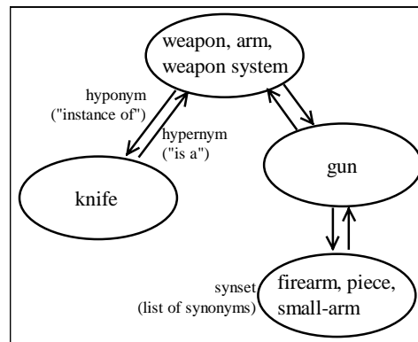
Figure 1: A piece of the WordNet semantic hierarchy (idealized model).
