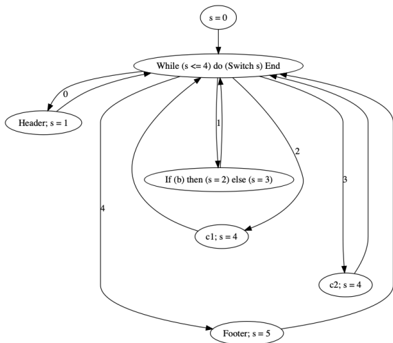
Figure 2. Flattened If-Then-Else
