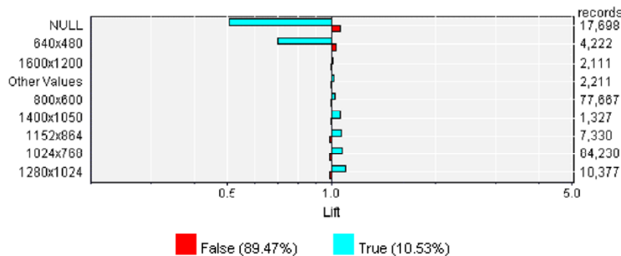
Figure 5: Lift chart showing relationship between screen resolution and search. NULL means the browser returned no information.
