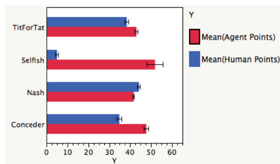
Figure 4: Average human and agent points in the end of the game per strategy (error bars denote 95% confidence intervals).
