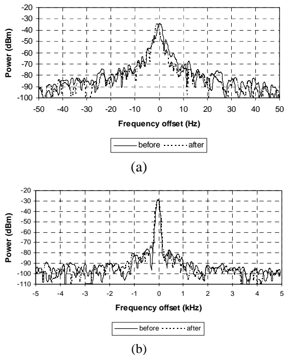
Fig. 14. Electrical spectra of the signal generated before and after transmission with dispersion compensation (a) Span of 100 Hz. (b) Span of 10 kHz.
