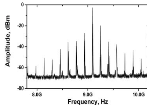
Fig. 5. Measured heterodyne beat-notes from two DFECLs [23].
