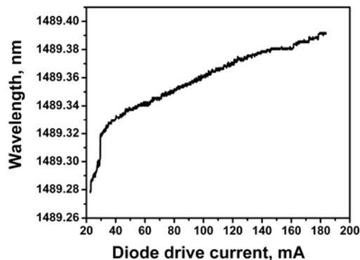
Fig. 4. Static chirp of the DFECL at 21°C [10].
