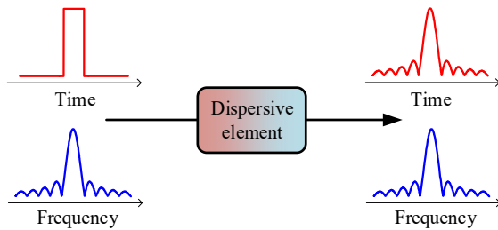
FIGURE 2. Schematic illustration of the frequency-to-time mapping.
