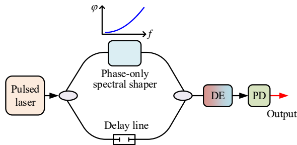
FIGURE 10. Chirped microwave waveform generation with a phase-only spectral shaper in a Mach-Zehnder interferometer (DE: dispersion element; PD: photodetector).
