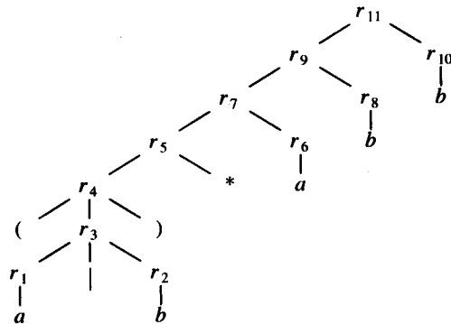
Fig. 3.30. Decomposition of (a|b)^*abb .
