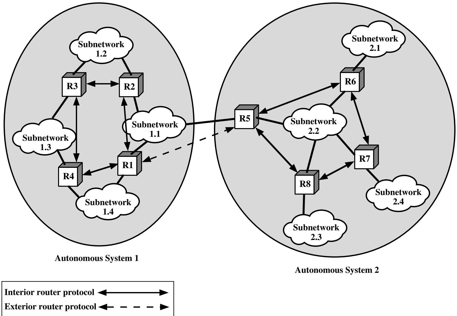
Figure 16.2 Application of Exterior and Interior Routing Protocols
