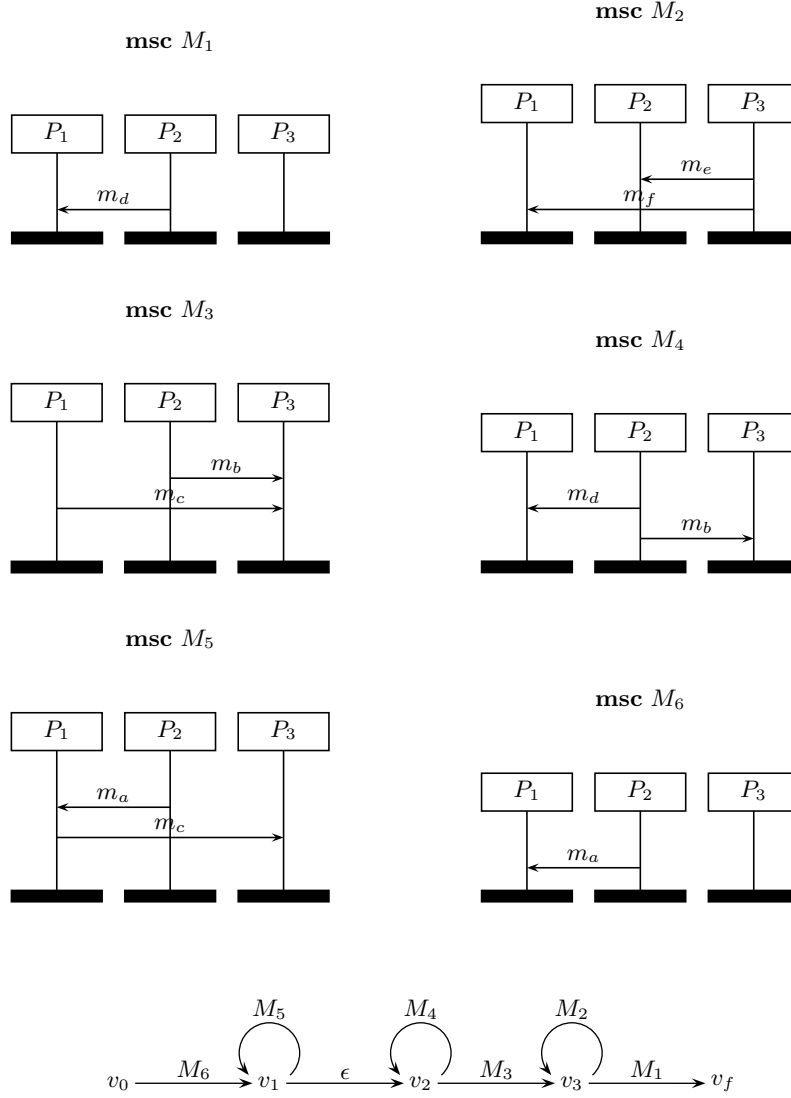
Fig. 3. Six MSCs obtained when processing M_{O_1} and M_{O_2} , and the final MSC-graph of the system as reverse engineered
