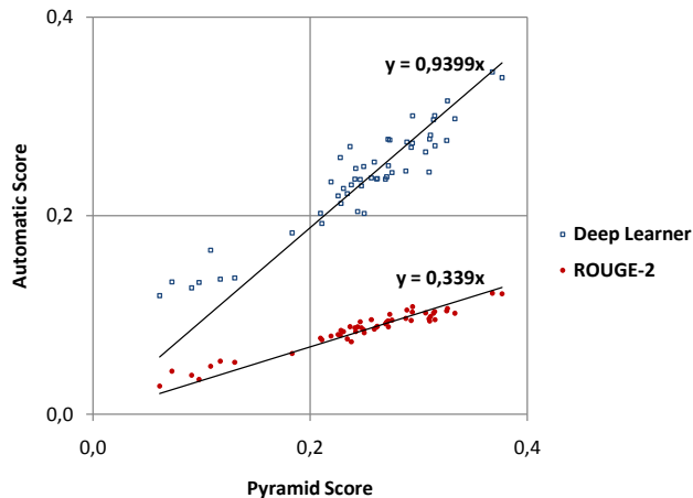
Fig. 4. Plot of averages of the predictions from our Deep Learning approach and ROUGE-2 against Pyramid scores, for each of the 52 evaluated systems.
