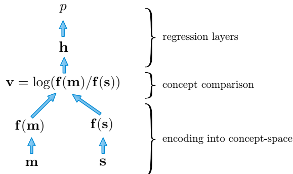
Fig. 2. Deep Learning architecture for regression, with three steps: encoding into concept-space, concept comparison and regression layers.
