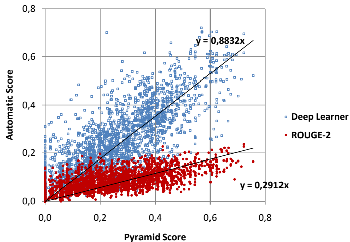
Fig. 3. Plot of the predictions from our Deep Learning approach and ROUGE-2 against Pyramid scores, for each of the 2288 summaries evaluated for testing. A large proportion of points have a Pyramid score of 0.
