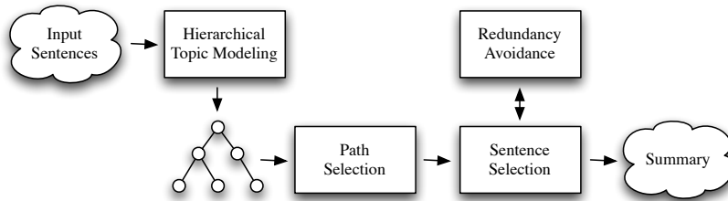
Fig. 1. The PathSum summarization framework.
