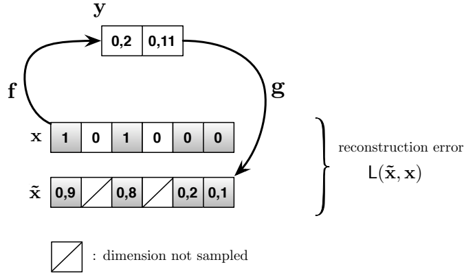
Fig. 1. Architecture of the auto-encoder to learn an encoding y in concept-space of an input x in term-space.
