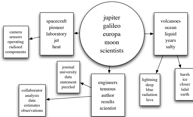
Fig. 2. A 3-level topic tree of the DUC 2006 document set describing NASA’s Galileo mission to Jupiter’s moons. The top 5 words in each topic are shown.
