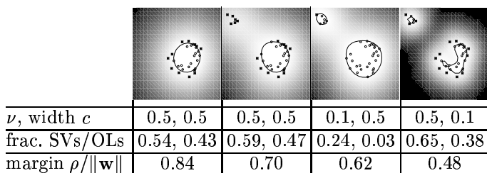
Fig. 14. A single-class SVM using RBF kernel (7) applied to a toy problem; domain: [-1, 1]^2 . First two pictures : Note how in both cases, at least a fraction of \nu of all examples is in the estimated region (cf. table). The large value of \nu causes the additional data points in the upper left corner to have almost no influence on the decision function. For smaller values of \nu , such as 0.1 ( third picture ), the points cannot be ignored anymore. Alternatively, one can force the algorithm to take these ‘outliers’ into account by changing the kernel width (7): in the fourth picture , using c = 0.1, \nu = 0.5 , the data is effectively analyzed on a different length scale which leads the algorithm to consider the outliers as meaningful points. Figure taken from [14].
