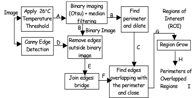
Fig. 2 System used to detect overlapping body parts
