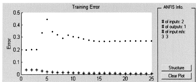
Fig. 8. Plot of the errors during the training of Go-Tangent-Oblique-Sensor ANFIS .
