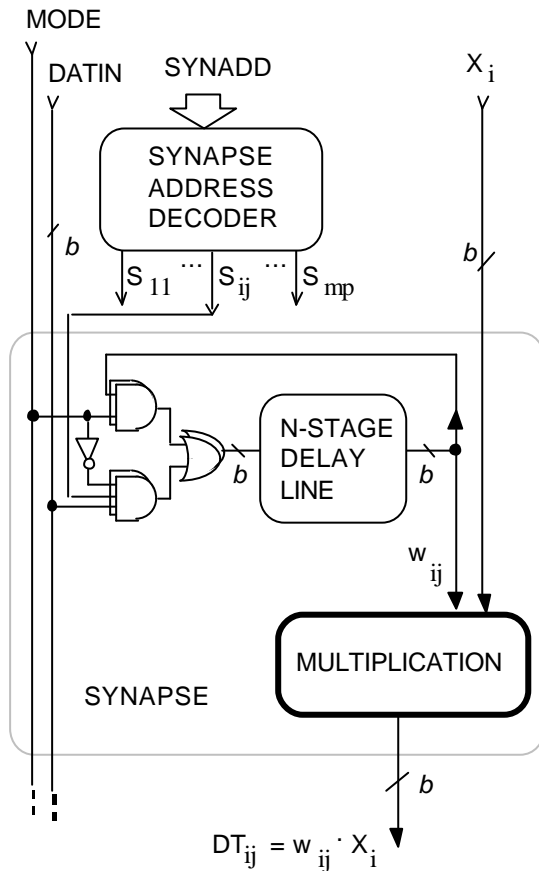
Multi-bit random-data implementation of a synapse
