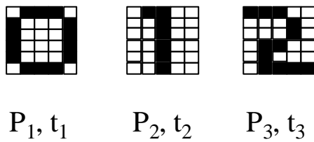
Training set
