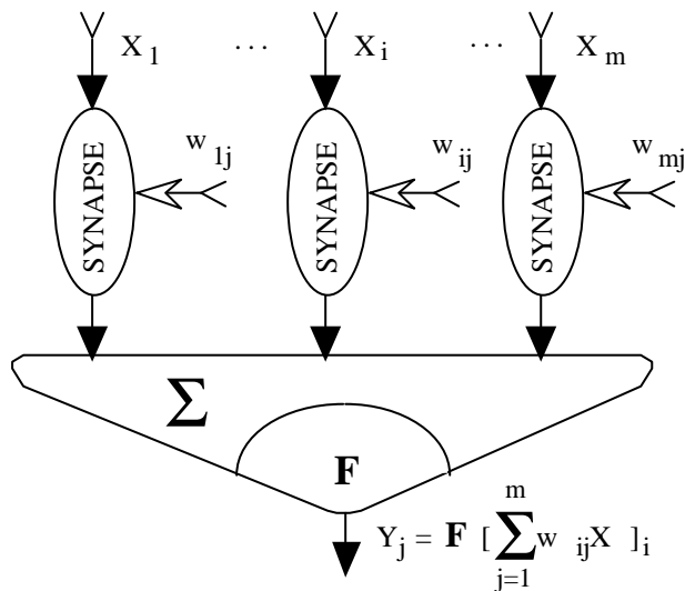
Neuron Structure
