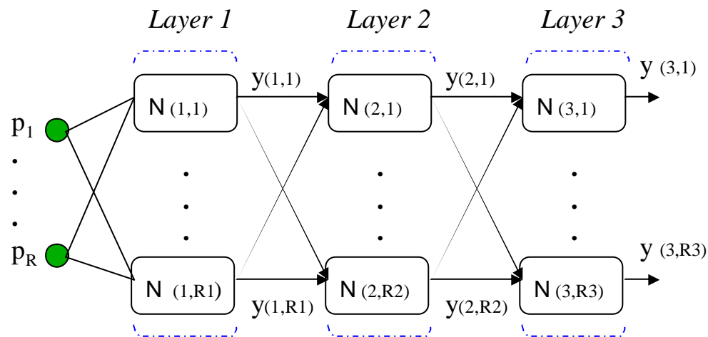
Feed-forward architecture with three layers
