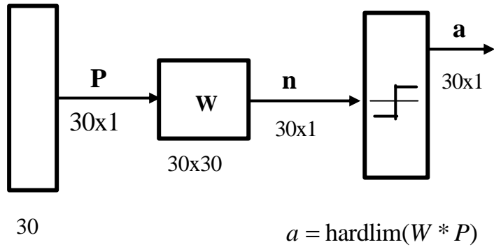
Auto-associative memory NN architecture
