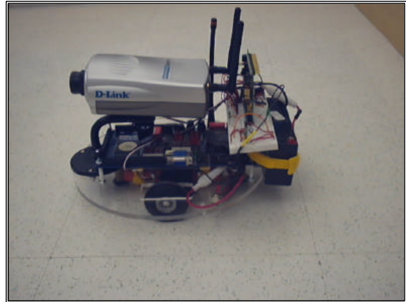
Two-wheel robotic platform for an experimental mobile autonomous robotic sensor agent equipped with a wireless camera, IR sensors and on computational power
