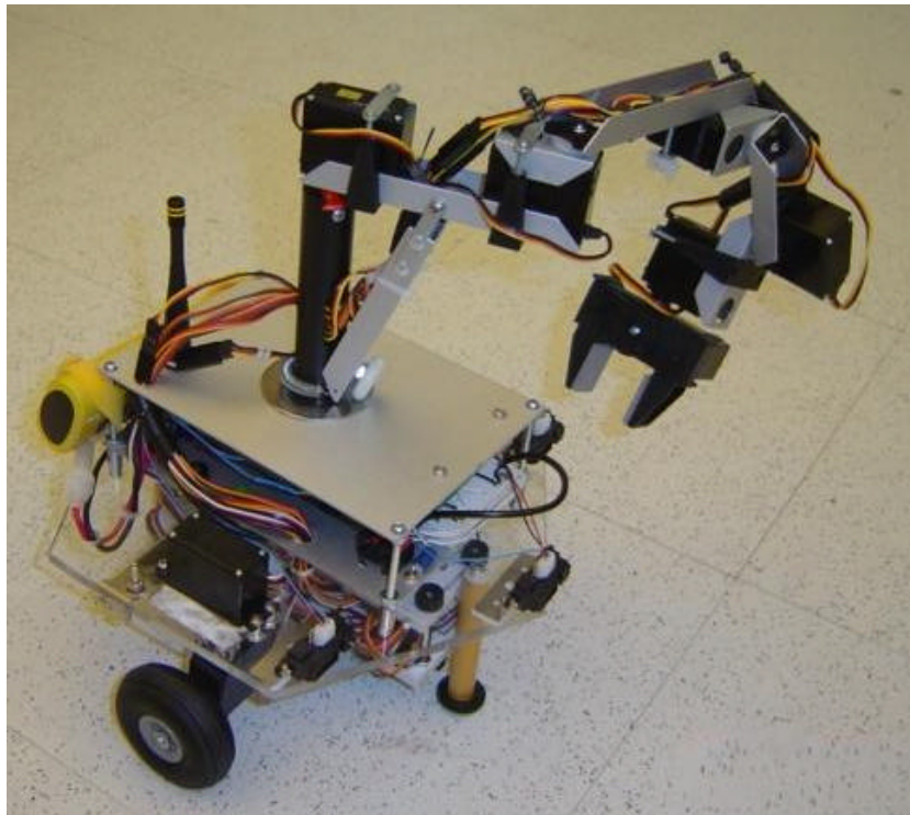
Two-wheeled hexagonal-shaped modular RSA platform equipped with onboard manipulator arm.
