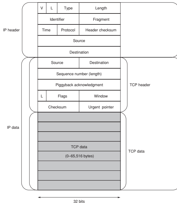
Figure E.35 The headers for IP and TCP. This drawing is 32 bits wide. The standard headers for both are 20 bytes, but both allow the headers to optionally lengthen for rarely transmitted information. Both headers have a length of header field (L) to accommodate the optional fields, as well as source and destination fields. The length field of the whole datagram is in a separate length field in IP, while TCP combines the length of the datagram with the sequence number of the datagram by giving the sequence number in bytes. TCP uses the checksum field to be sure that the datagram is not corrupted, and the sequence number field to be sure the datagrams are assembled into the proper order when they arrive. IP provides checksum error detection only for the header, since TCP has protected the rest of the packet. One optimization is that TCP can send a sequence of datagrams before waiting for permission to send more. The number of datagrams that can be sent without waiting for approval is called the window , and the window field tells how many bytes may be sent beyond the byte being acknowledged by this datagram. TCP will adjust the size of the window depending on the success of the IP layer in sending datagrams; the more reliable and faster it is, the larger TCP makes the window. Since the window slides forward as the data arrive and are acknowledged, this technique is called a sliding window protocol . The piggyback acknowledgment field of TCP is another optimization. Since some applications send data back and forth over the same connection, it seems wasteful to send a datagram containing only an acknowledgment. This piggyback field allows a datagram carrying data to also carry the acknowledgment for a previous transmission, “piggybacking” on top of a data transmission. The urgent pointer field of TCP gives the address within the datagram of an important byte, such as a break character. This pointer allows the application software to skip over data so that the user doesn’t have to wait for all prior data to be processed before seeing a character that tells the software to stop. The identifier field and fragment field of IP allow intermediary machines to break the original datagram into many smaller datagrams. A unique identifier is associated with the original datagram and placed in every fragment, with the fragment field saying which piece is which. The time-to-live field allows a datagram to be killed off after going through a maximum number of intermediate switches no matter where it is in the network. Knowing the maximum number of hops that it will take for a datagram to arrive—if it ever arrives—simplifies the protocol software. The protocol field identifies which possible upper layer protocol sent the IP datagram; in our case, it is TCP. The V (for version) and type fields allow different versions of the IP protocol software for the network. Explicit version numbering is included so that software can be upgraded gracefully machine by machine, without shutting down the entire network. In 2006, version six of the Internet protocol (IPv6) was widely used.
