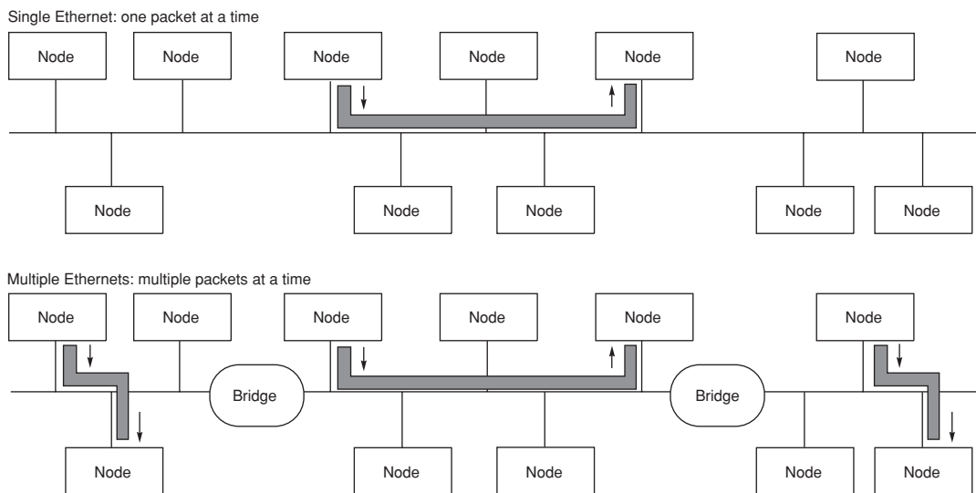
Figure E.30 The potential increased bandwidth of using many Ethernets and bridges.
