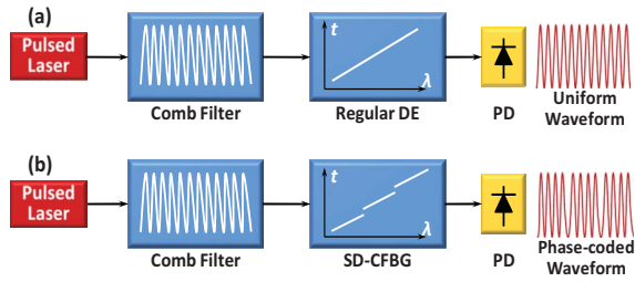
Fig. 1. Microwave waveform generation based on spectral pulse shaping and frequency-to-time mapping. (a) A uniform microwave pulse is generated using a regular dispersive element (DE) and (b) a phase-coded microwave pulse is generated using a SD-CFBG with discrete time delay jumps.
