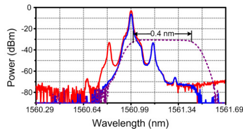
Fig. 2. Optical single-sideband signal generation using an optical filter with a passband having steep edges and a flat top. Dash line: the transmission spectrum of the optical filter; red line: the optical spectrum of the ODSB signal; and blue line: the optical spectrum of the generated OSSB signal.
