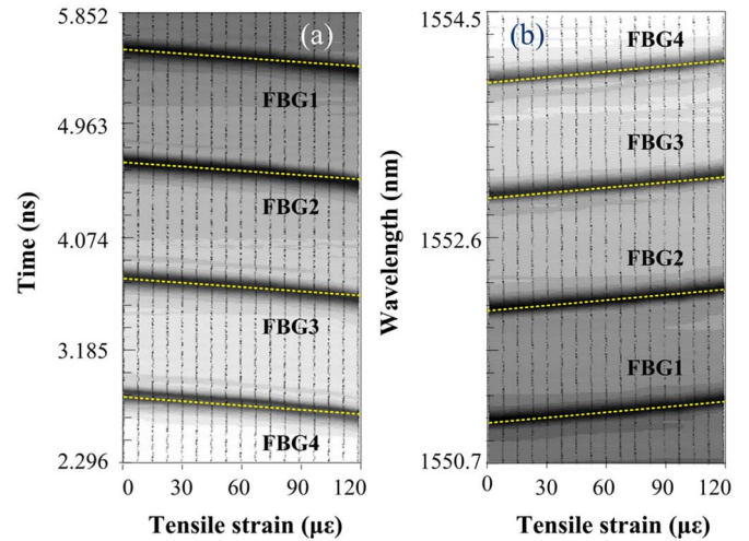
Fig. 7. (a) Contour map of the temporal waveforms and (b) contour map the spectra in the wavelength domain obtained from (a) using (18).
