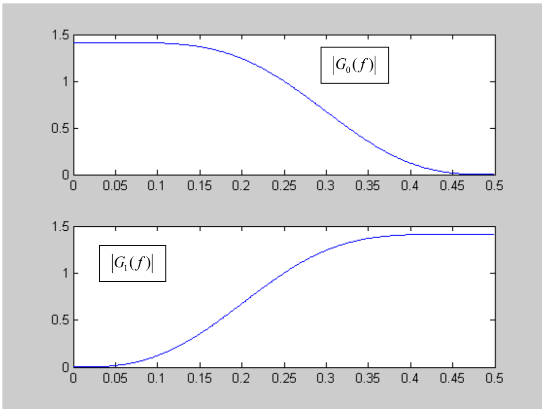
Magnitude frequency response of two channels
