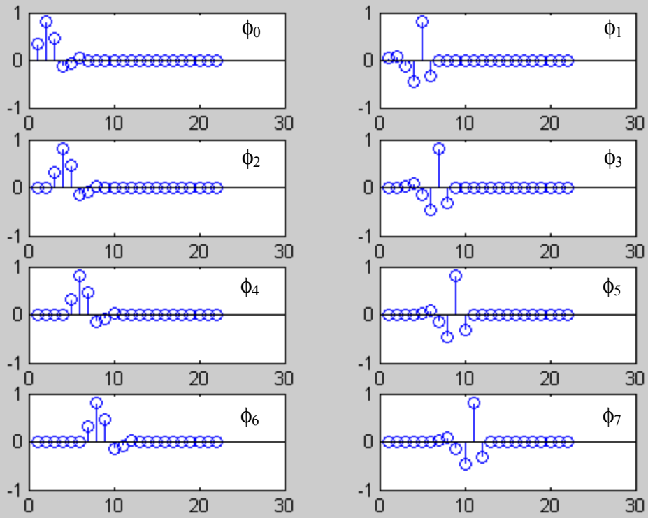
Two-channel filter-bank Orthonormal basis
