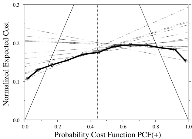
Figure 7. Credit: Over-sampling, Disabling Pruning
