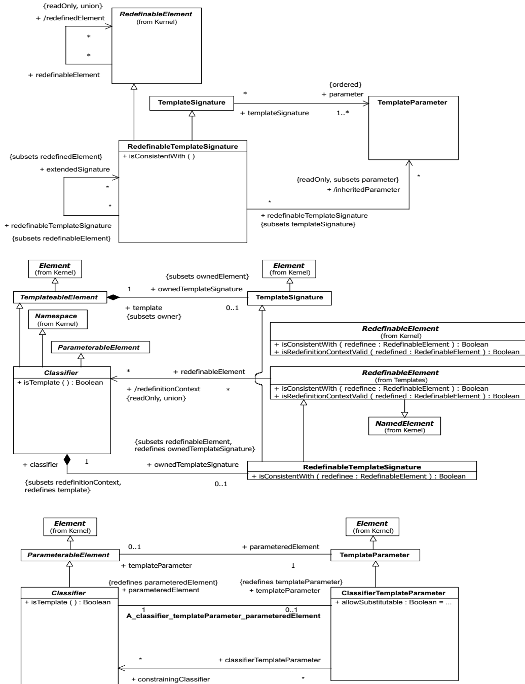
Figure 17.13 - Classifier templates
