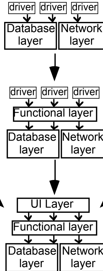
Bottom-up testing
