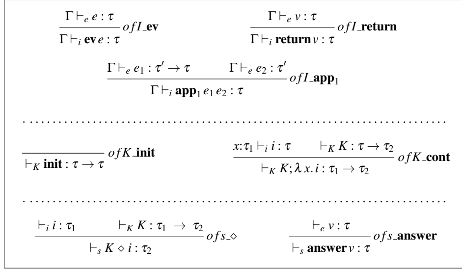
Figure 11: Typing rules for the continuation machine
