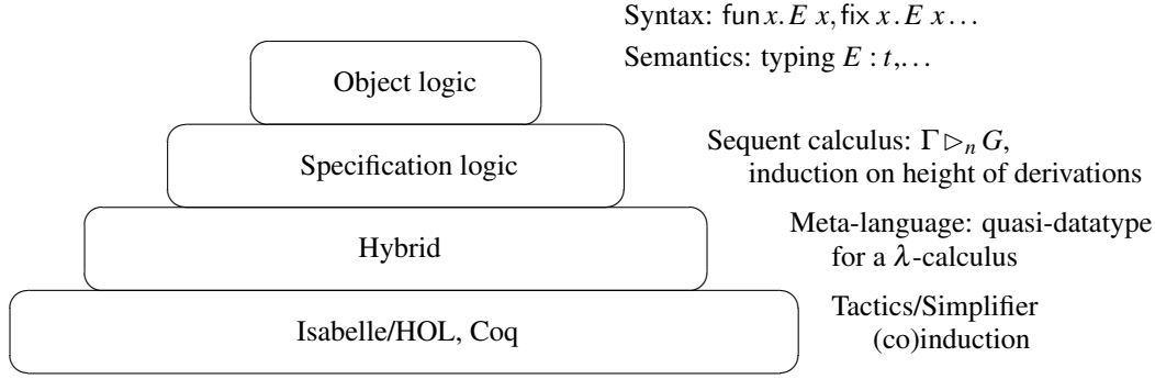
Figure 1: Architecture of the Hybrid system
