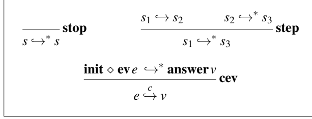
Figure 10: Top level transition rules
