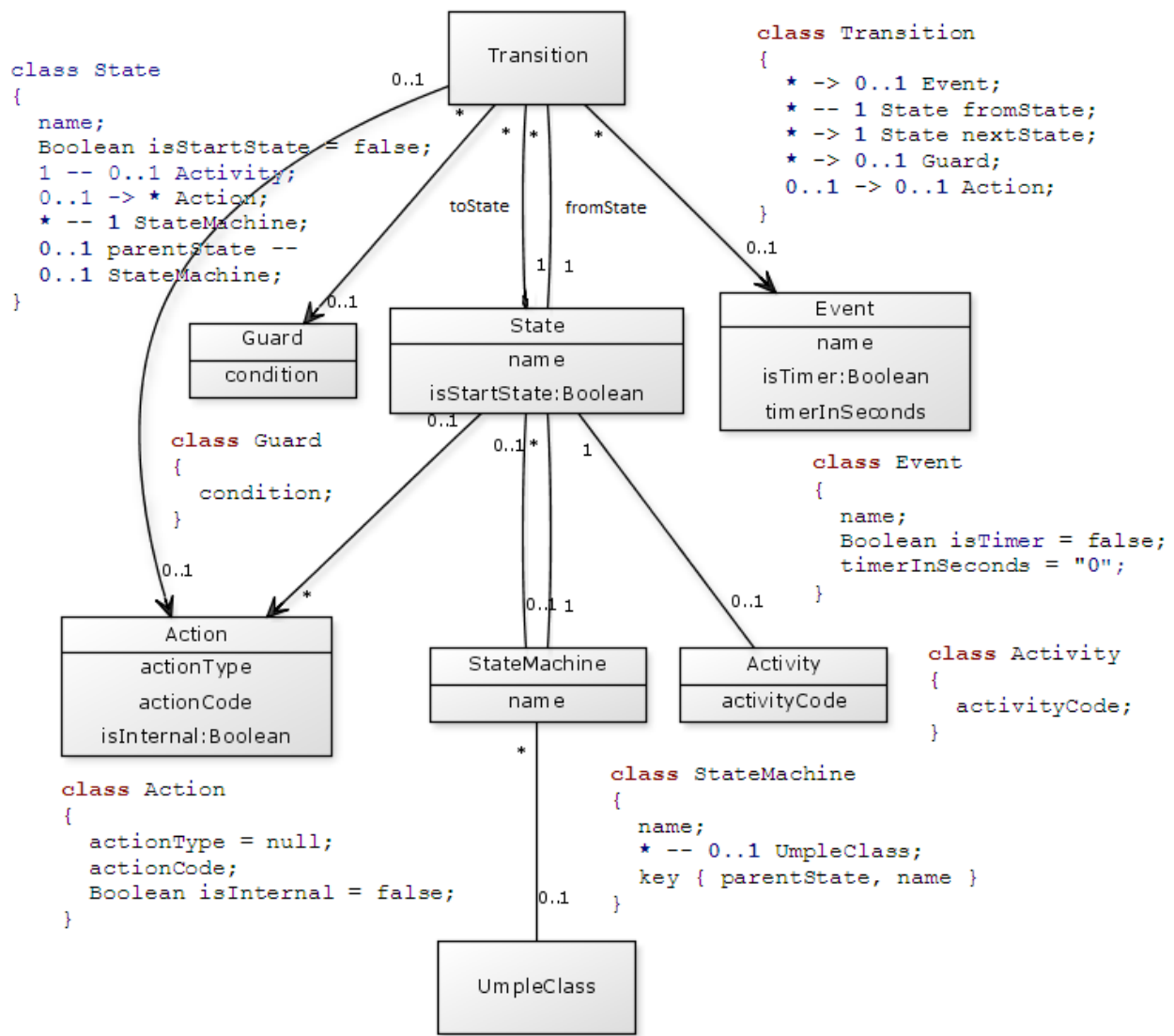
Figure 12: Umple meta-model
