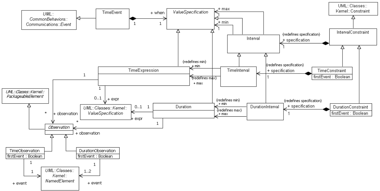
Figure 13.13 - SimpleTime
