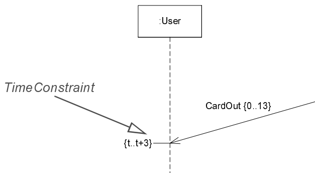
Figure 13.17 - TimeConstraint
