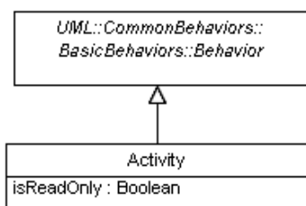
Figure 12.7 - Elements
