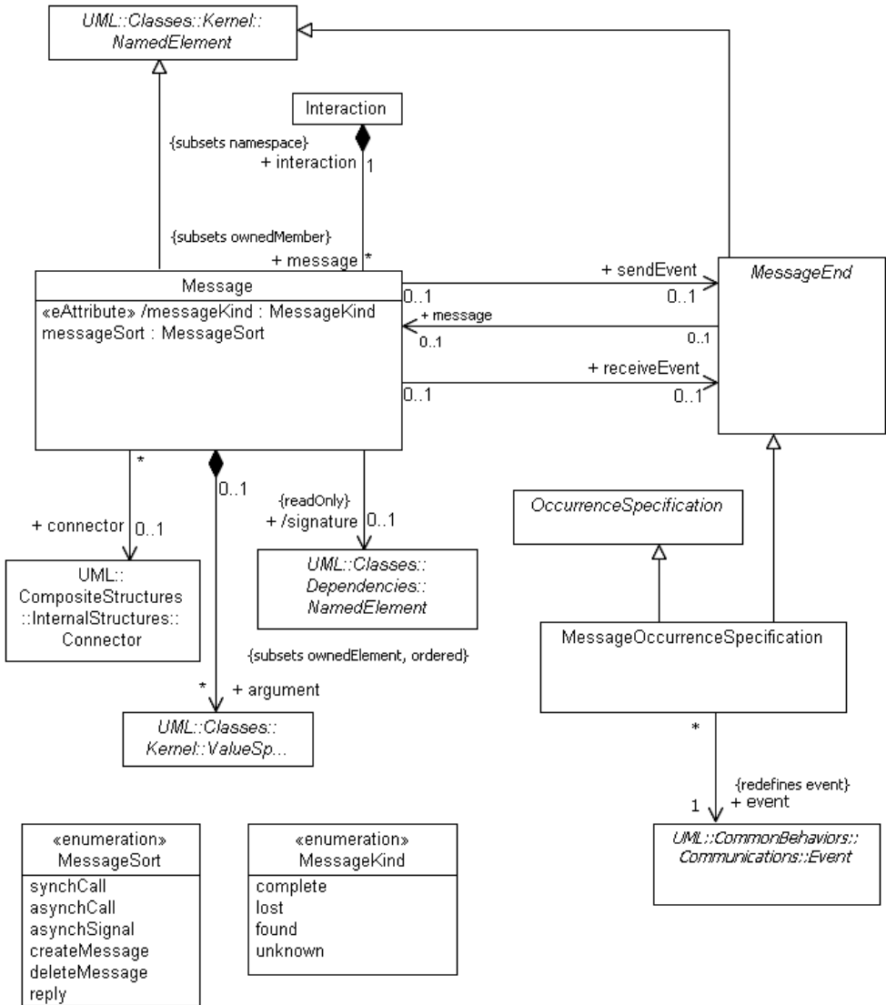
Figure 14.5 - Messages
