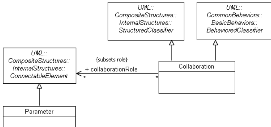
Figure 9.6 - Collaboration
