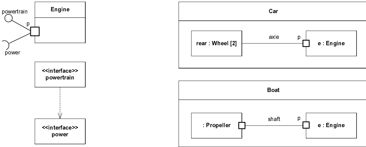
Figure 9.19 - Port examples
