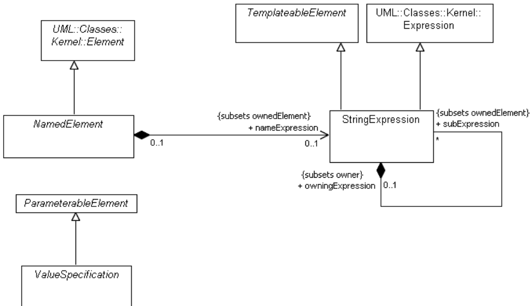
Figure 17.27 - Name expression
