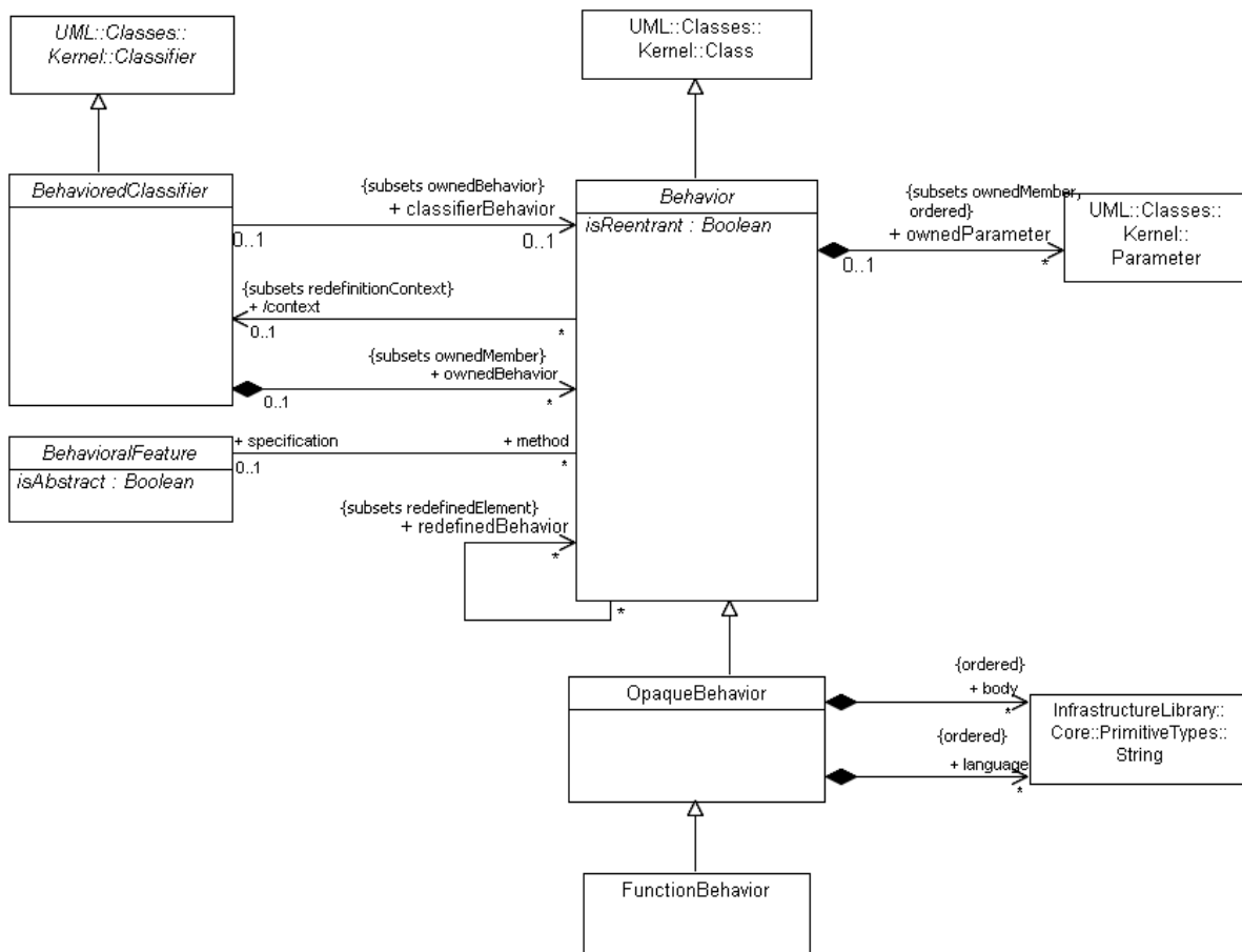
Figure 13.6 - Common Behavior
