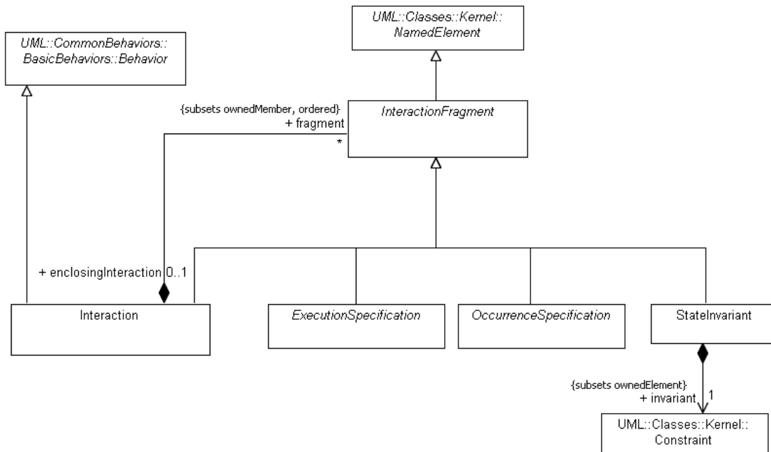
Figure 14.3 - Interactions
