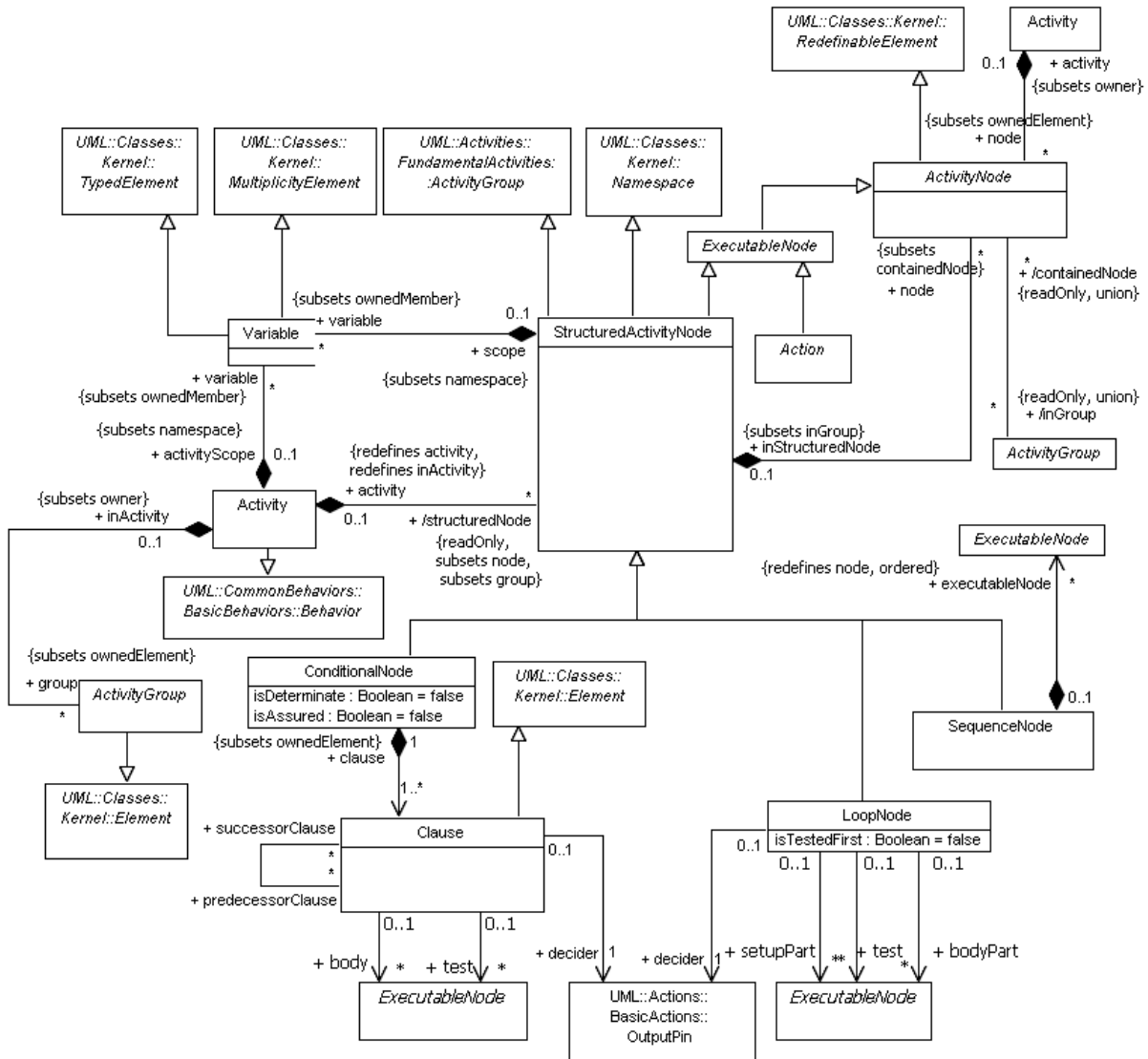
Figure 12.21 - Structured nodes
