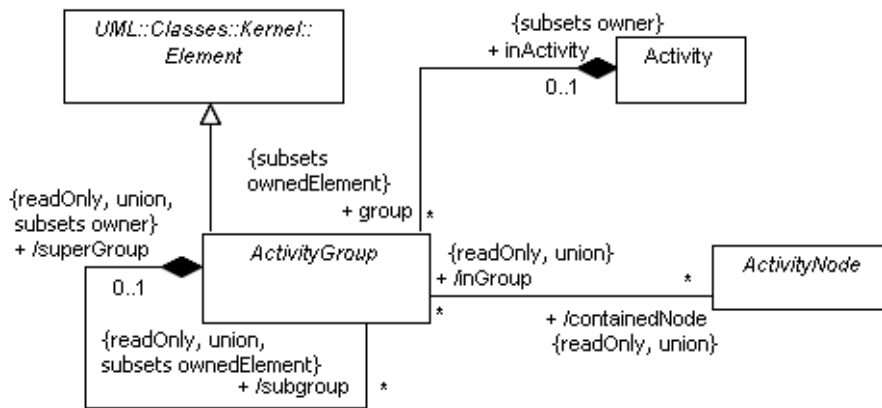
Figure 12.3 - Fundamental groups
