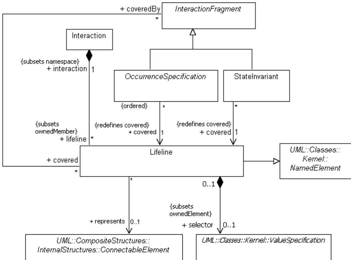
Figure 14.4 - Lifelines
