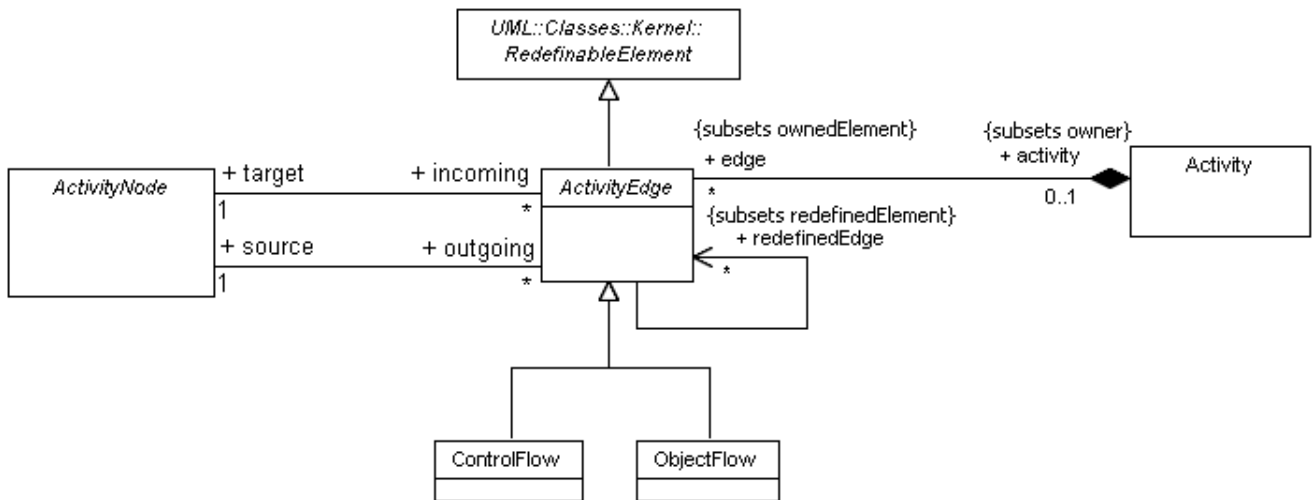
Figure 12.5 - Flows
