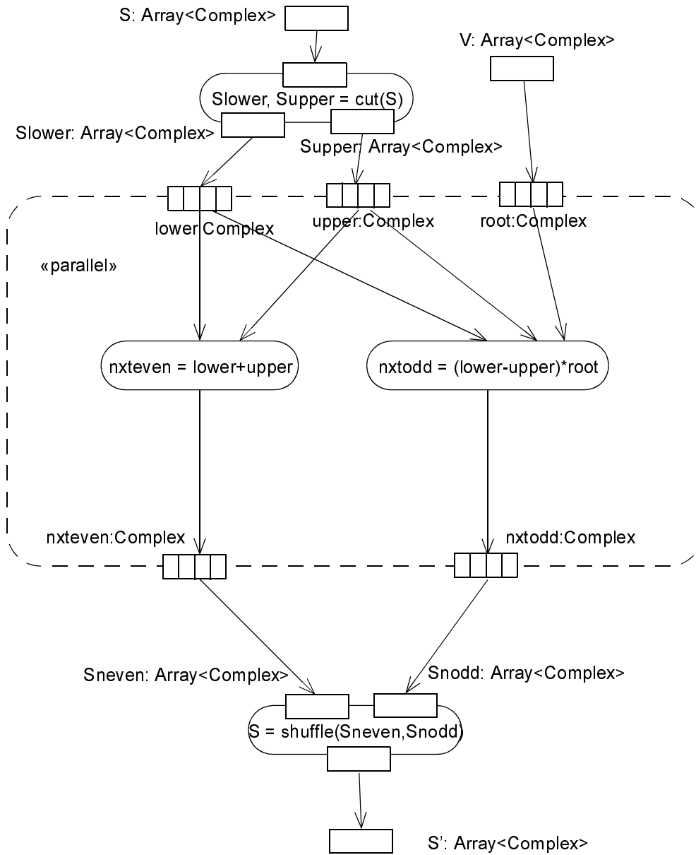
Figure 12.87 - Expansion region
