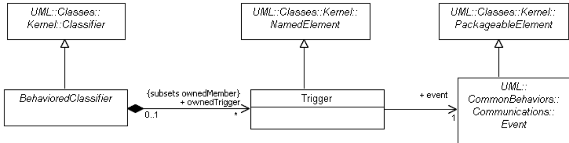
Figure 13.11 - Triggers
