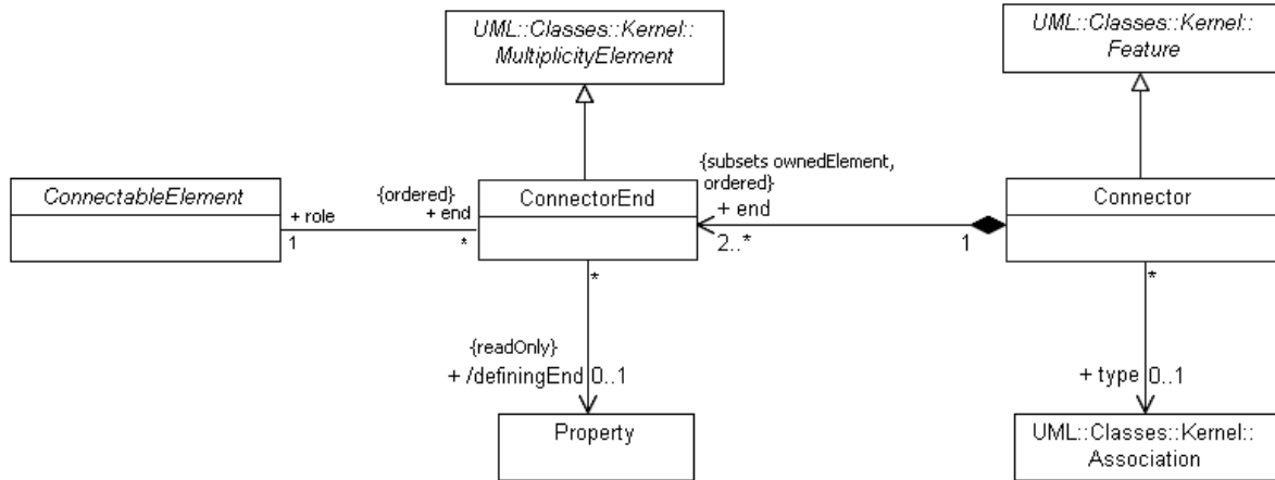
Figure 9.3 - Connectors
