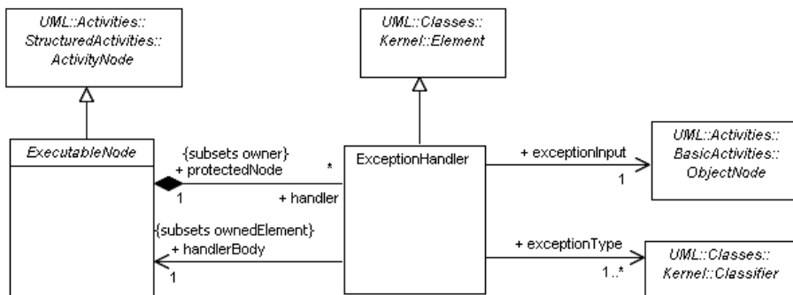
Figure 12.23 - Exceptions
