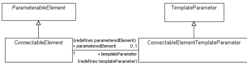
Figure 17.30 - Connectable element template parameters
