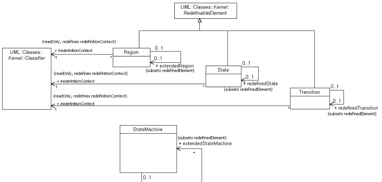
Figure 15.3 - State Machine Redefinitions
