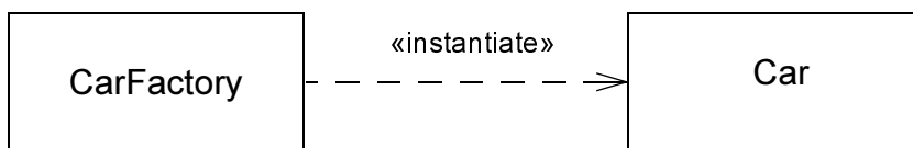
Figure 7.38 - An example of an instantiate dependency
