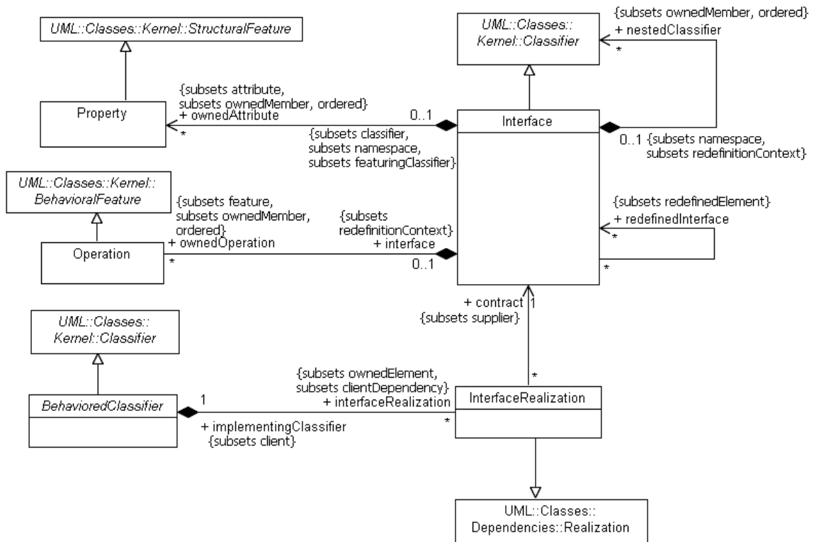
Figure 7.16 - Contents of Interfaces package
