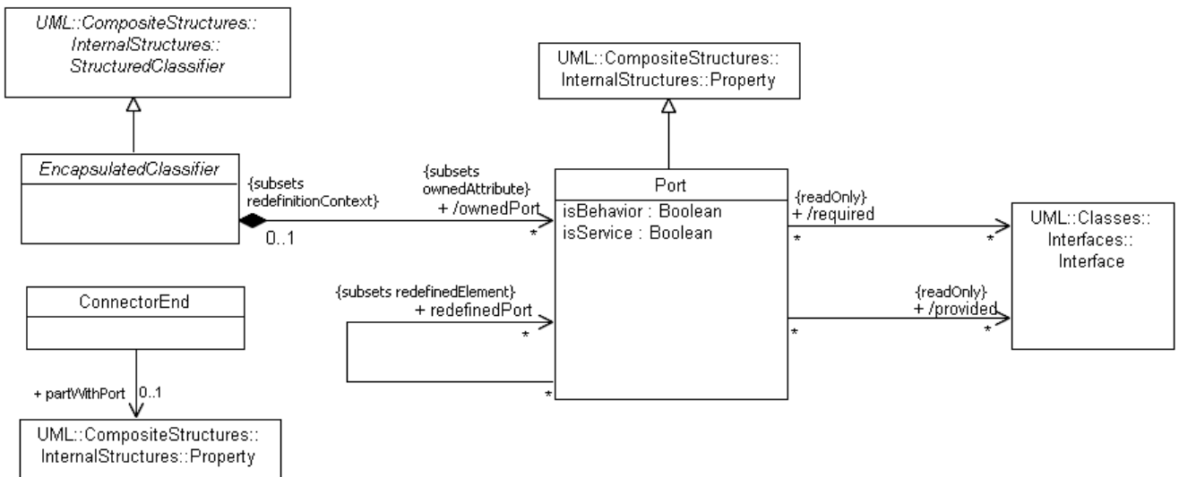
Figure 9.4 - The Port metaclass
