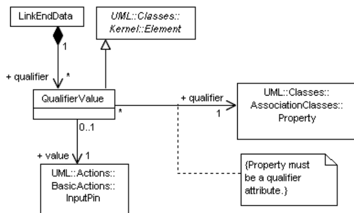
Figure 11.14 - Link identification (CompleteActions)
