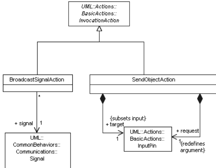
Figure 11.5 - Intermediate invocation actions
