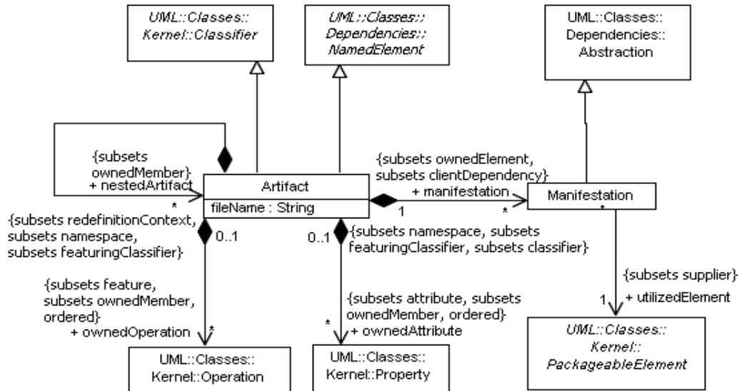
Figure 10.2 - The elements defined in the Artifacts package
