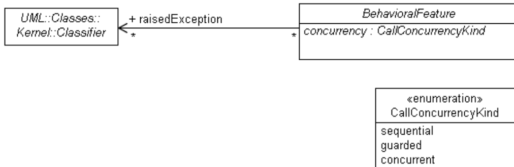
Figure 13.10 - Extensions to behavioral features
