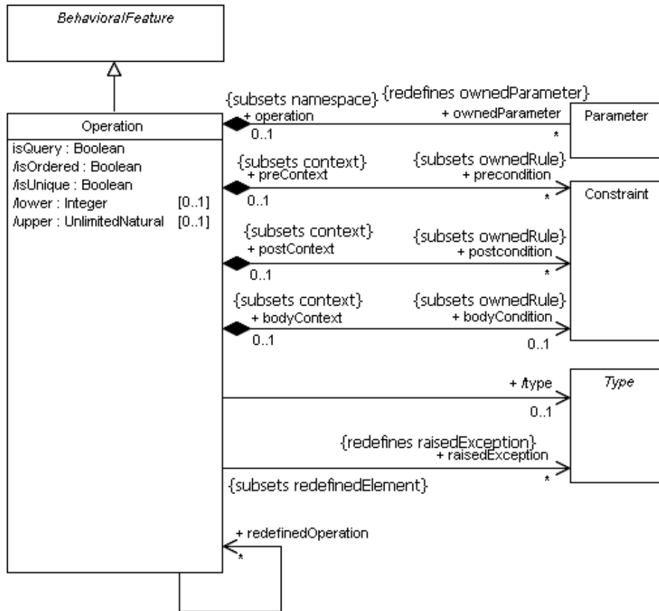
Figure 7.11 - Operations diagram of the Kernel package
