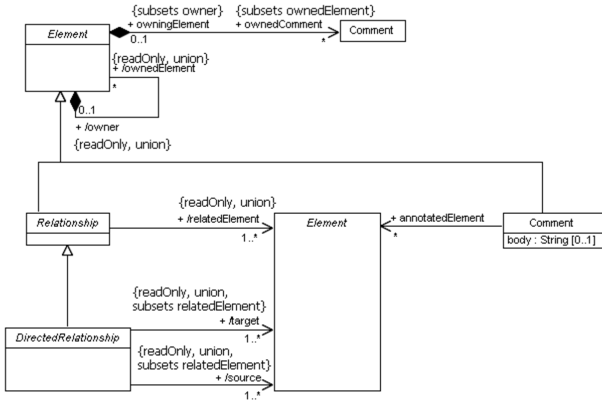
Figure 7.3 - Root diagram of the Kernel package
