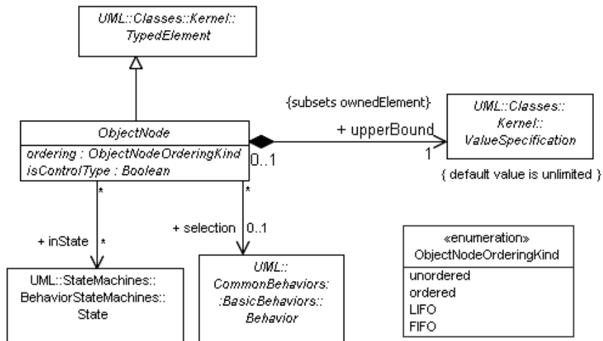
Figure 12.15 - Object nodes (CompleteActivities)
