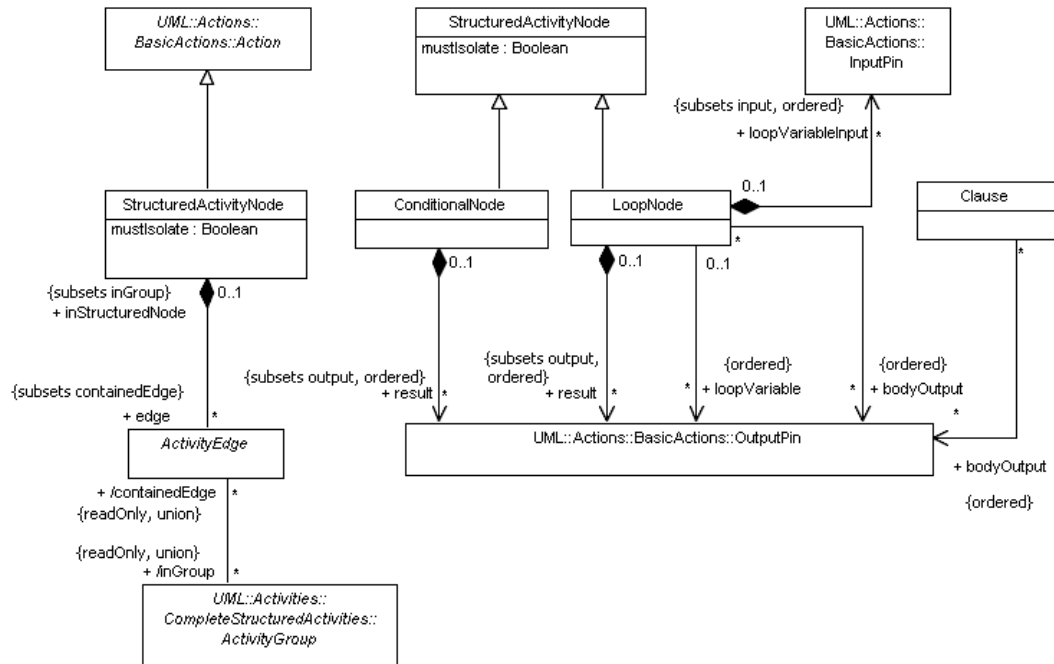
Figure 12.22 - Structured nodes ( CompleteStructuredActivities )
