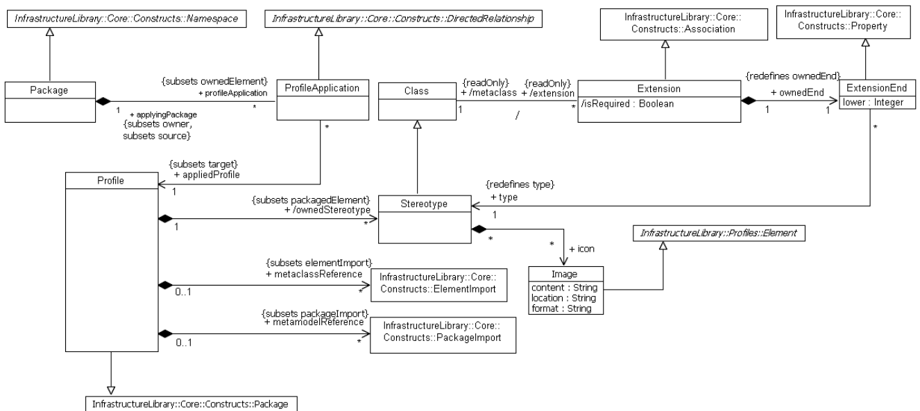
Figure 18.2 - The elements defined in the Profiles package
