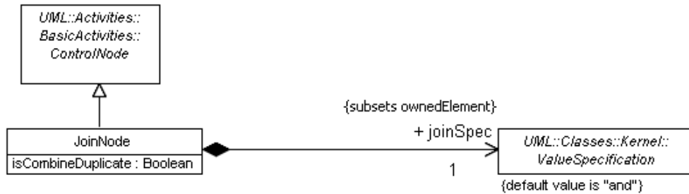
Figure 12.19 - Control nodes (CompleteActivities)
