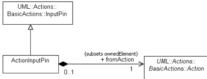
Figure 11.20 - Action input pin
