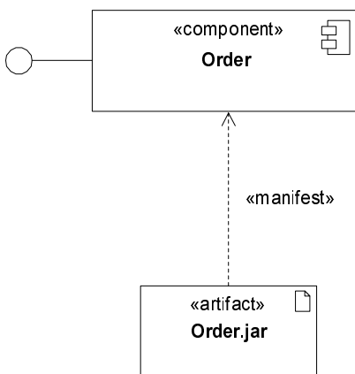
Figure 10.6 - An Artifact instance
