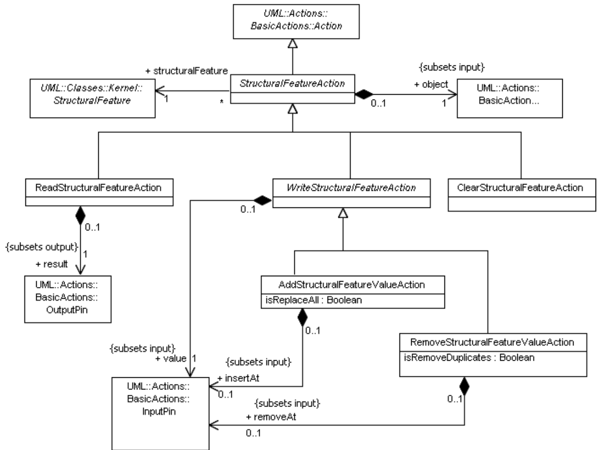
Figure 11.7 - Structural Feature Actions
