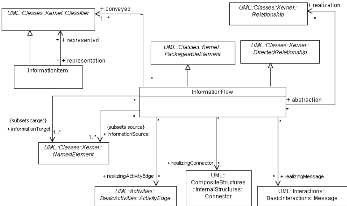
Figure 17.2 - The contents of the InformationFlows package
