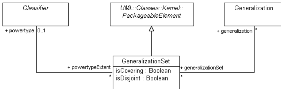
Figure 7.18 - Contents of PowerTypes package
