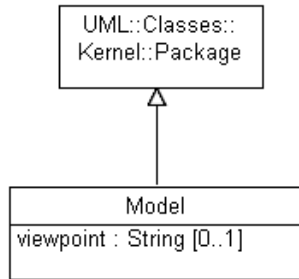
Figure 17.8 - The contents of the Models package
