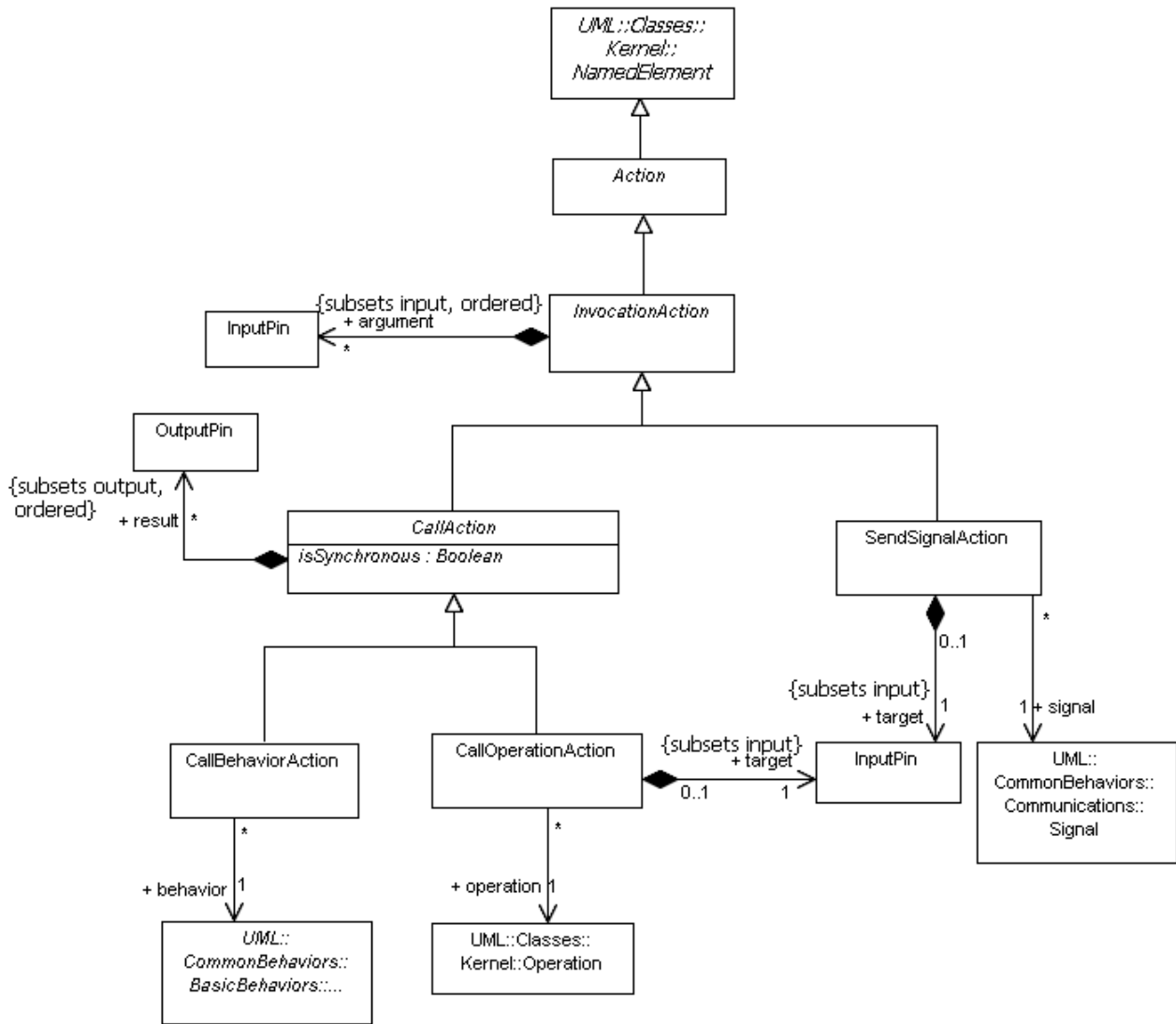
Figure 11.4 - Basic invocation actions
