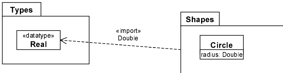
Figure 7.40 - Example of element import with aliasing
