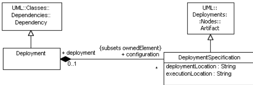
Figure 10.5 - Metaclasses that define component Deployment
