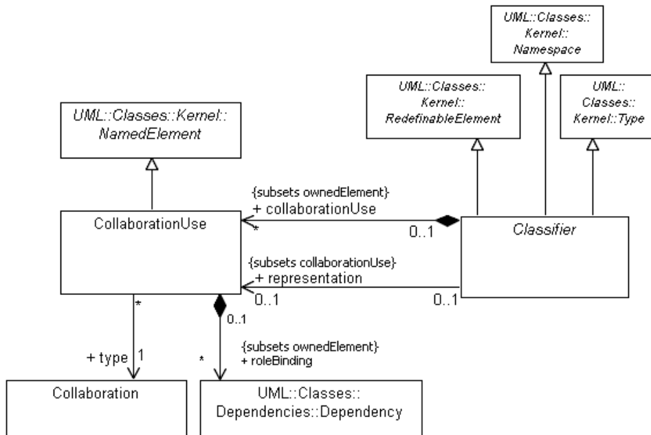
Figure 9.7 - Collaboration.use and role binding
