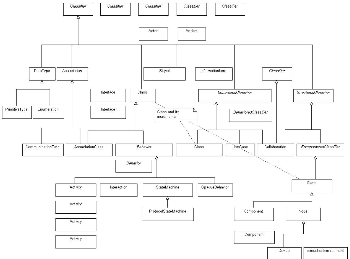
Figure F.1 - Classifier hierarchy for UML 2.0 Superstructure
