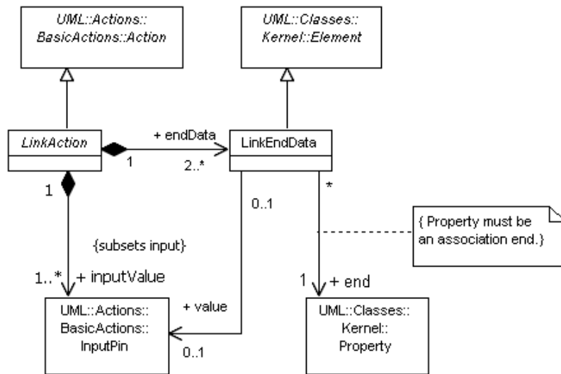
Figure 11.8 - Link identification
