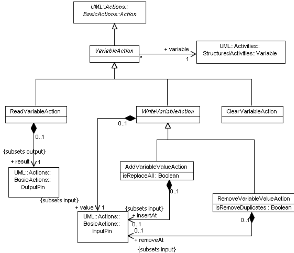
Figure 11.18 - Variable actions
