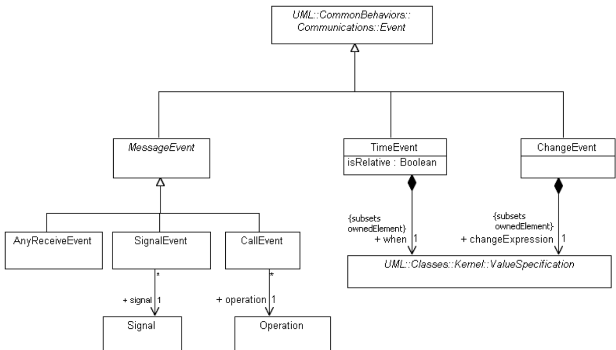
Figure 13.12 - Events
