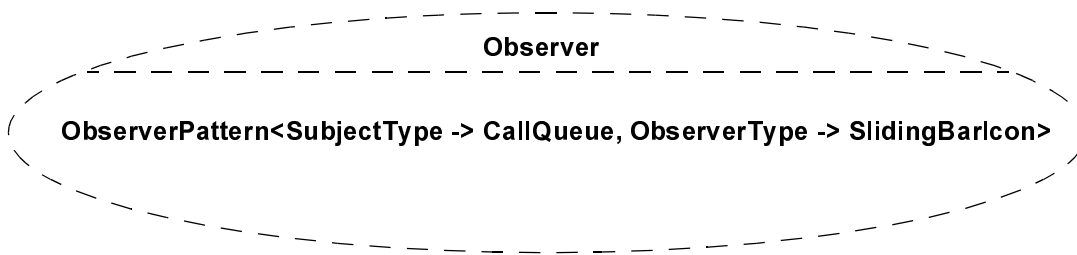
Figure 17.24 - Bound Collaboration
