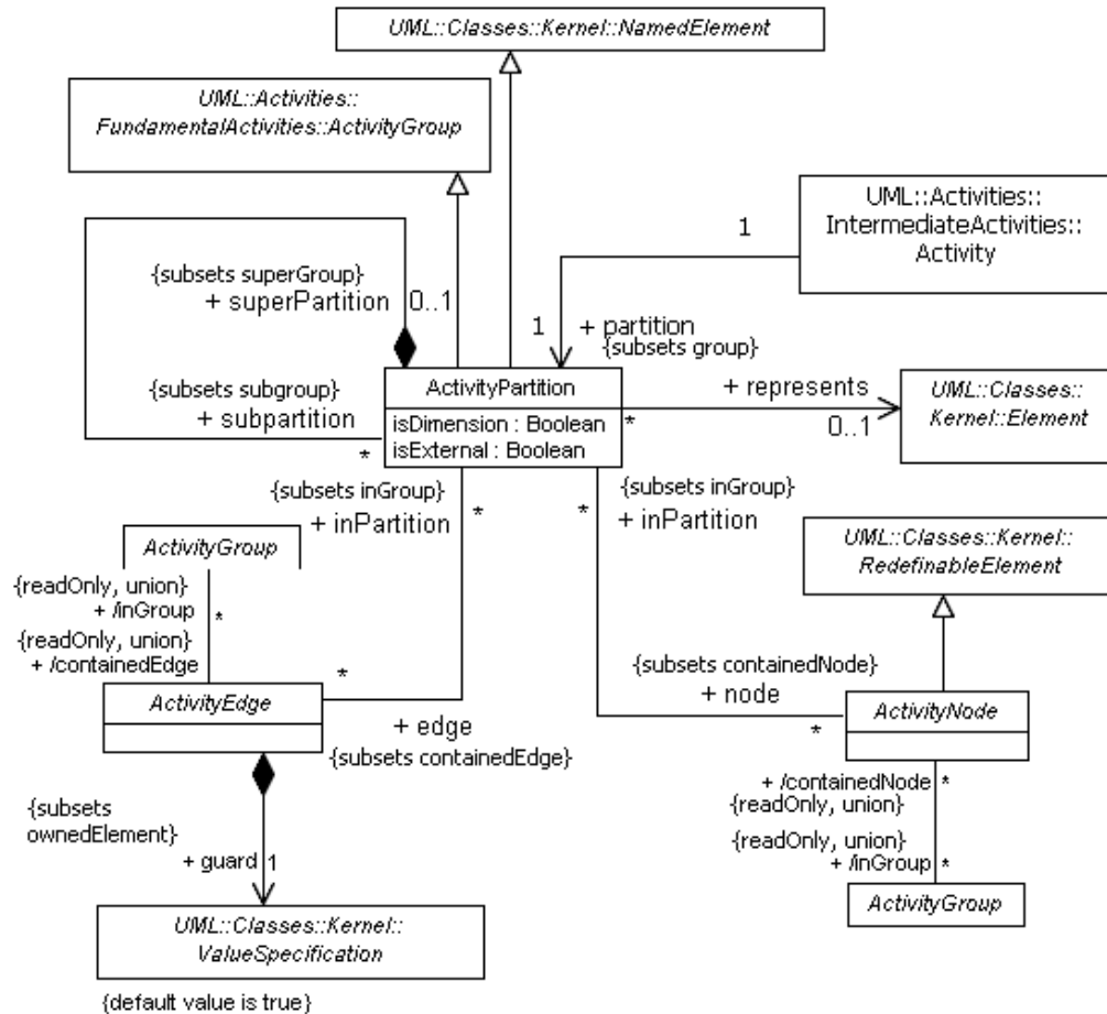
Figure 12.10 - Partitions
