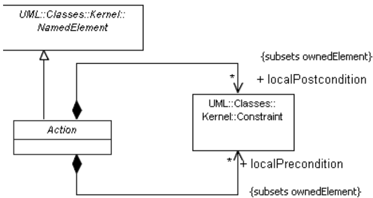
Figure 12.13 - Constraints (CompleteActivities)
