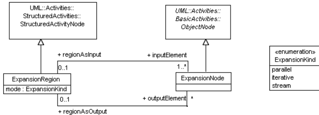
Figure 12.24 - Expansion regions
