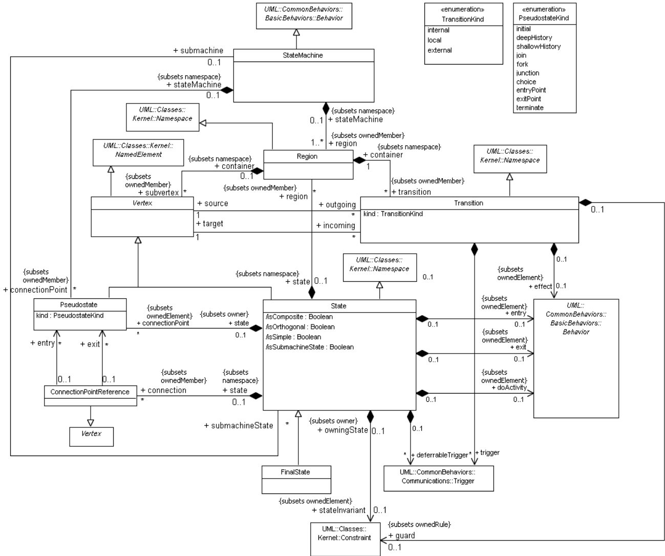
Figure 15.2 - State Machines
