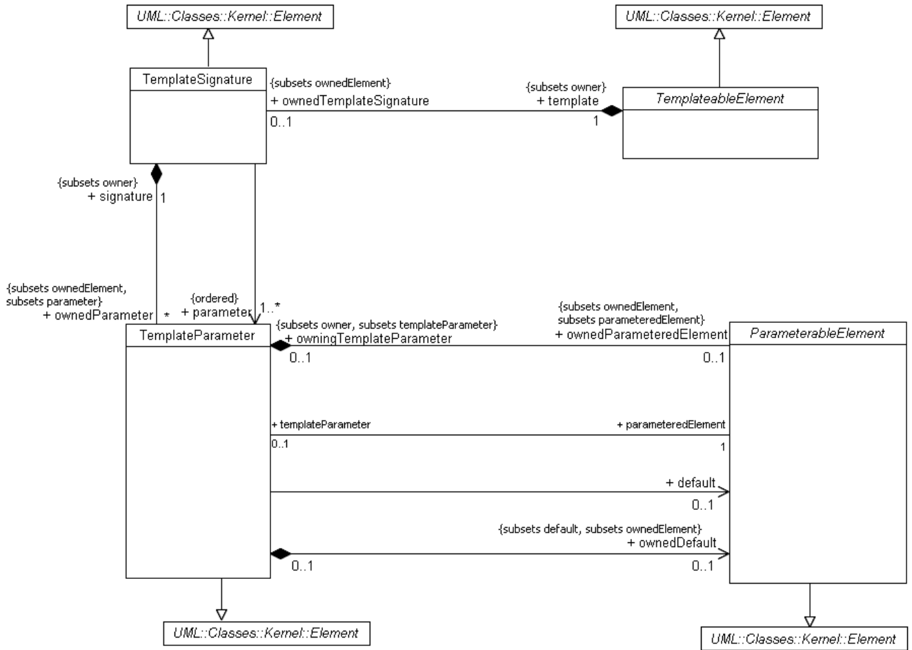
Figure 17.16 - Templates
