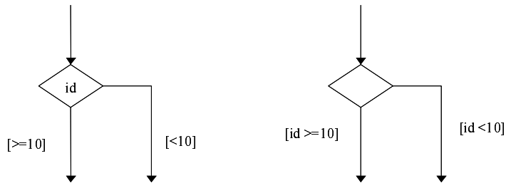
Figure 15.23 - Choice Pseudostate
