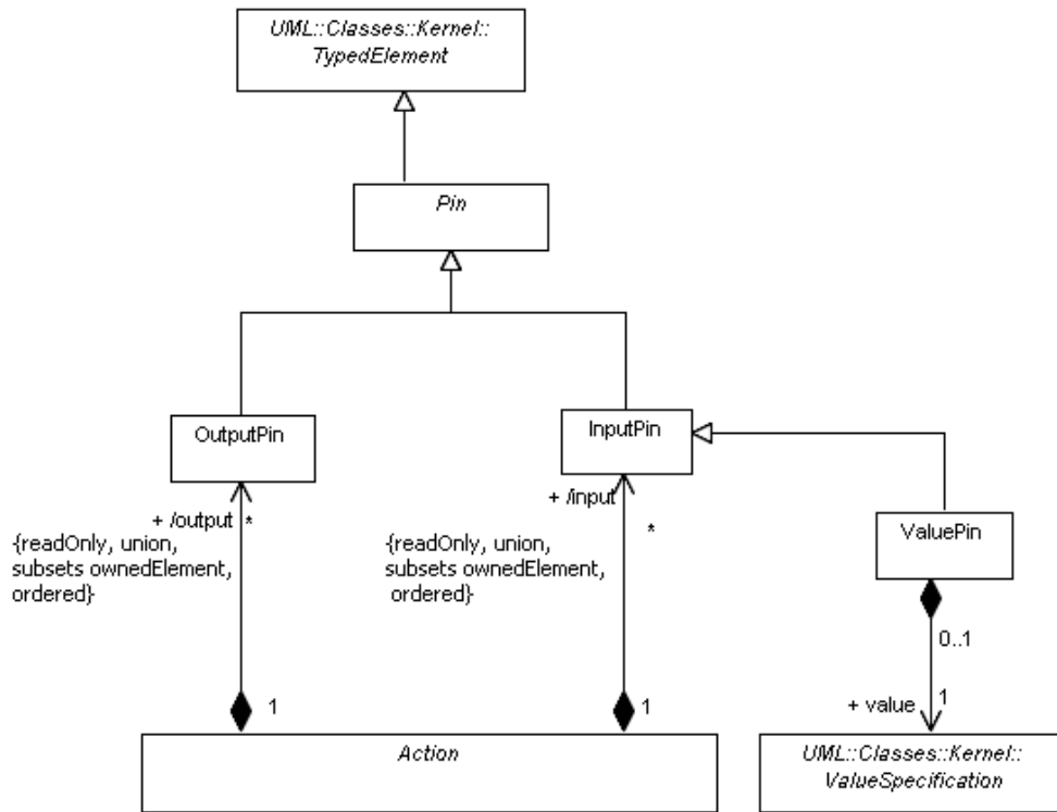
Figure 11.3 - Basic pins
