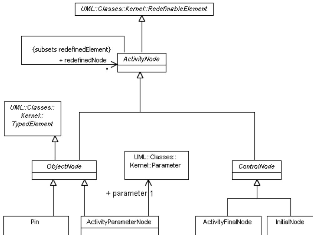
Figure 12.4 - Nodes (BasicActivities)
