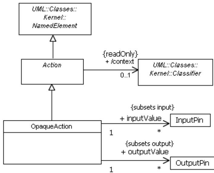
Figure 11.2 - Basic actions
