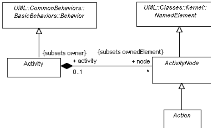
Figure 12.2 - Fundamental nodes
