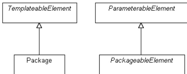
Figure 17.25 - Package templates
