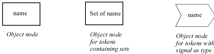
Figure 12.114 - Object node notations
