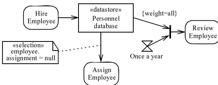
Figure 12.75 - Data store node example
