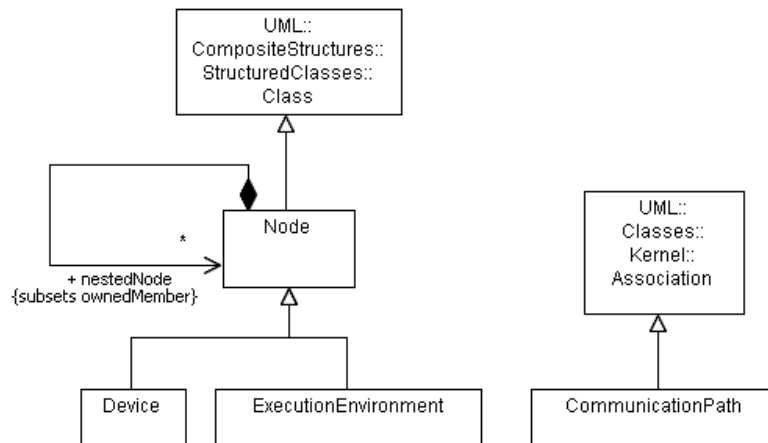
Figure 10.3 - The definition of the Node concept
