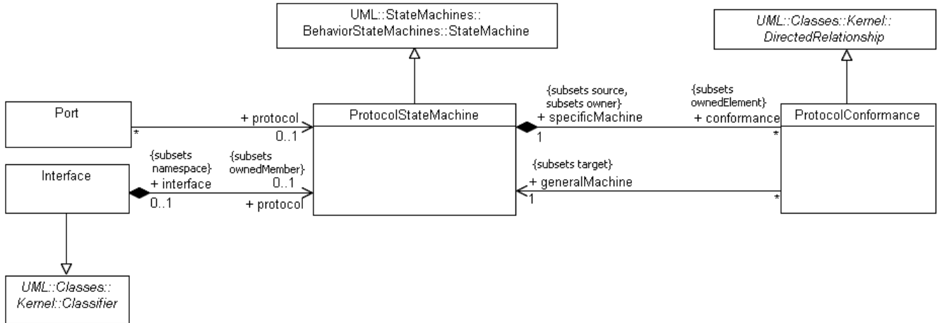
Figure 15.5 - Protocol State Machines
