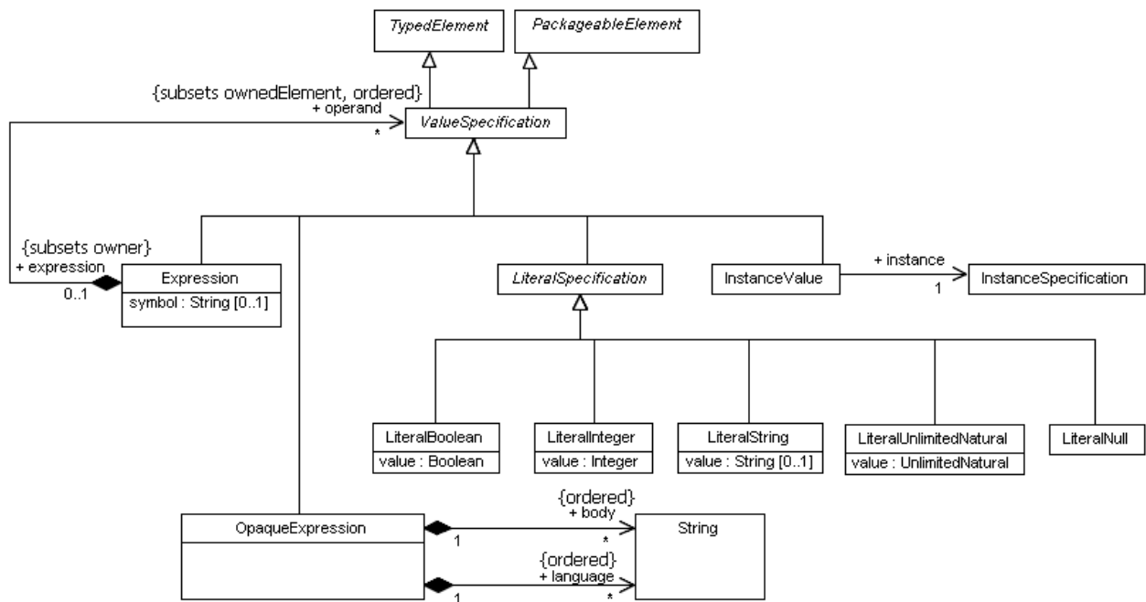
Figure 7.6 - Expressions diagram of the Kernel package
