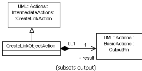
Figure 11.16 - Write link actions (CompleteActions)
