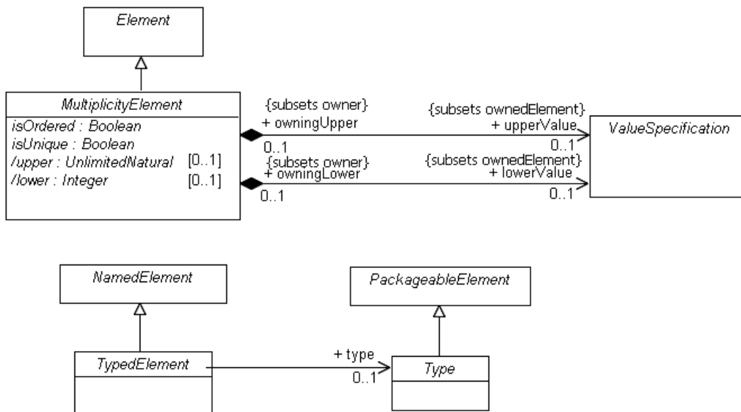
Figure 7.5 - Multiplicities diagram of the Kernel package
