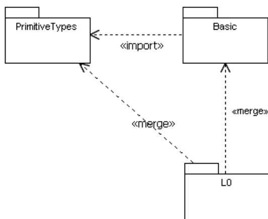
Figure 2.1 - Level 0 package diagram
