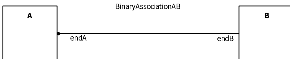
Figure 7.19 - Graphic notation indicating exactly one association end owned by the association
