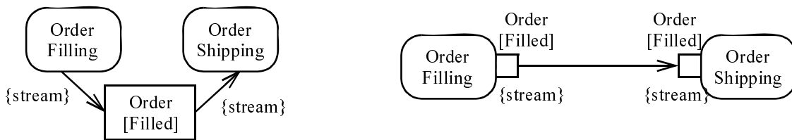
Figure 12.128 - Pin examples
