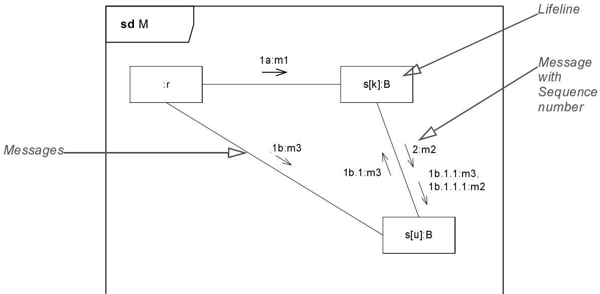
Figure 14.27 - Communication diagram
