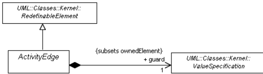
Figure 12.11 - Flows (IntermediateActivities)
