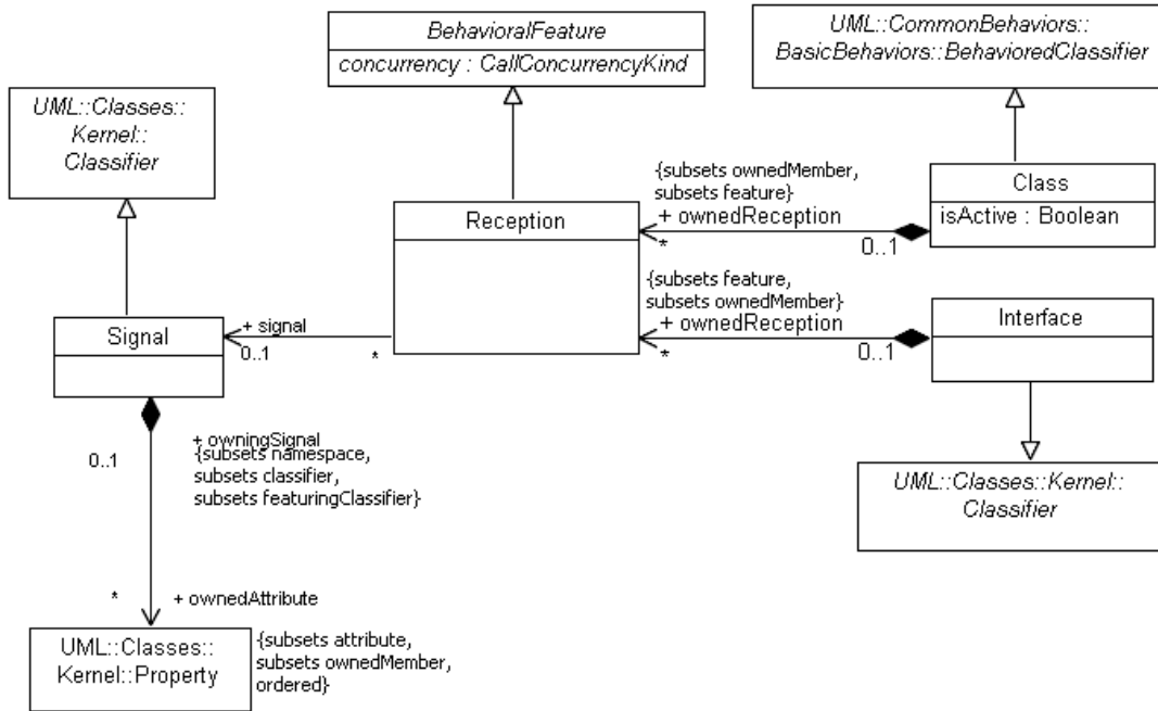
Figure 13.9 - Reception
