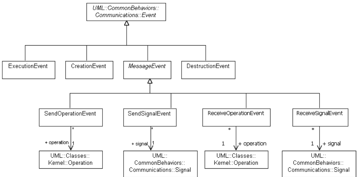
Figure 14.2 Events
