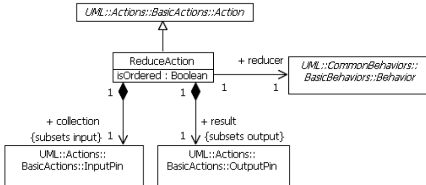
Figure 11.17 - ReduceAction (CompleteActions)
