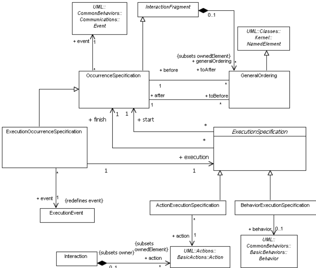
Figure 14.6 Occurrences
