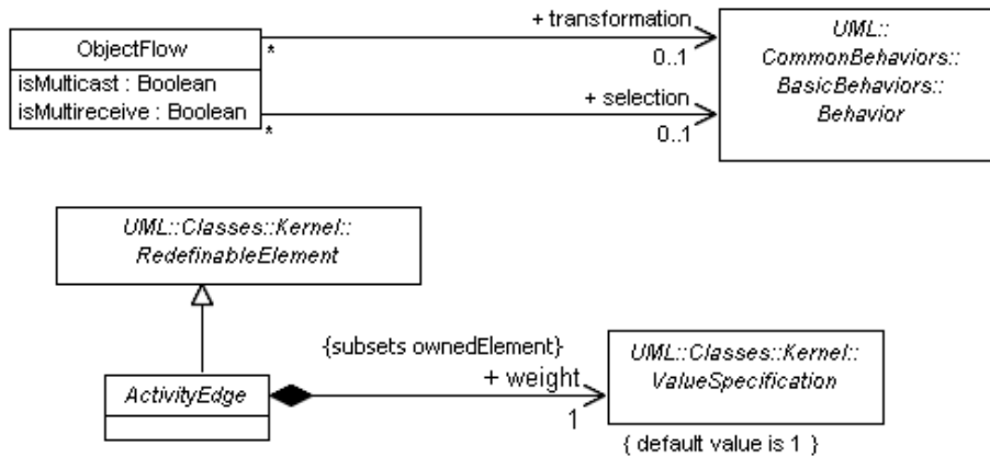
Figure 12.14 - Flows (CompleteActivities)
