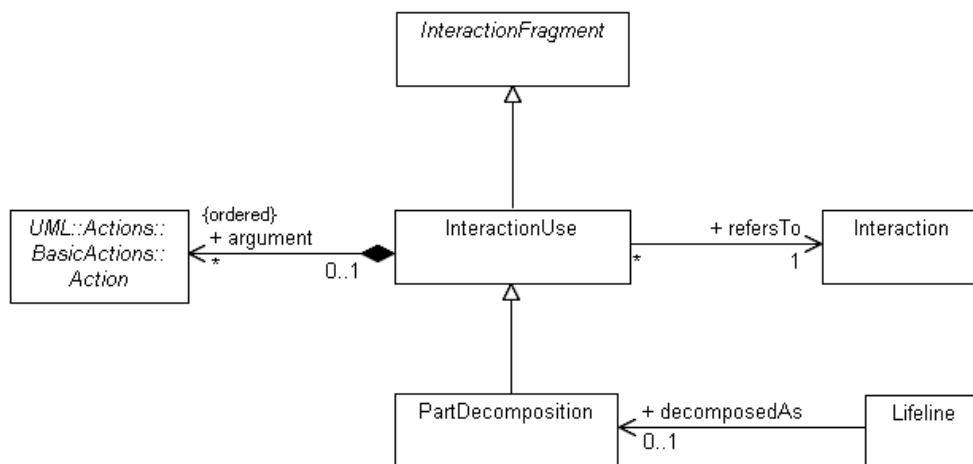
Figure 14.9 - InteractionUses
