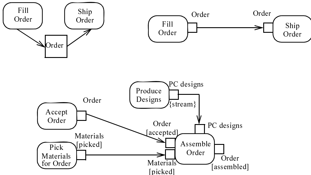
Figure 12.126 - Pin examples
