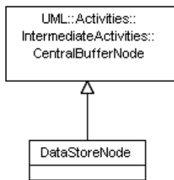
Figure 12.17 - Data stores
