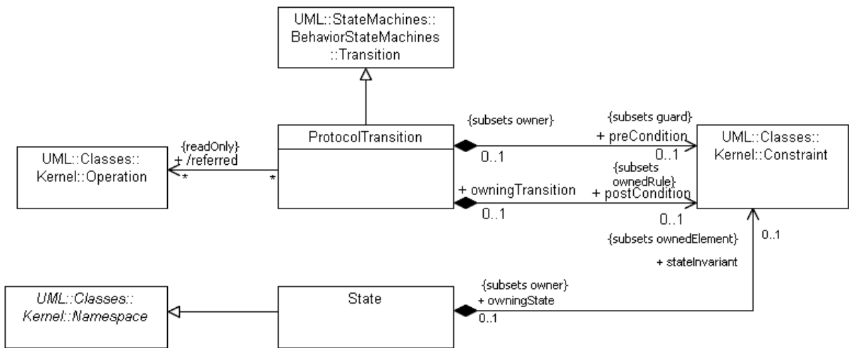
Figure 15.6 - Constraints
