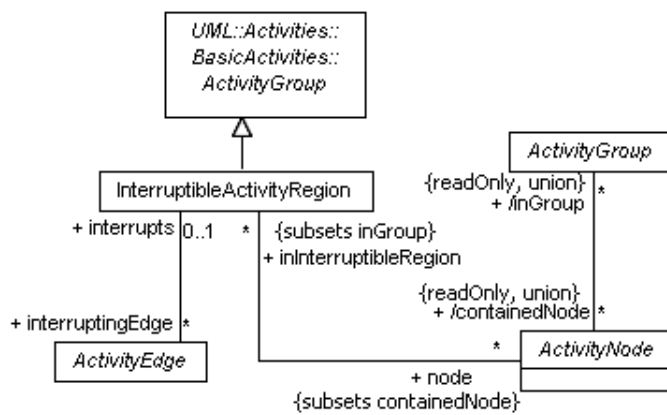
Figure 12.20 - Interruptible regions
