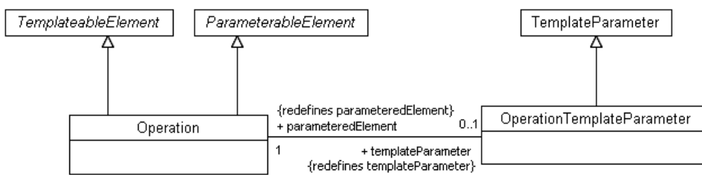
Figure 17.29 - Operation templates and parameters
