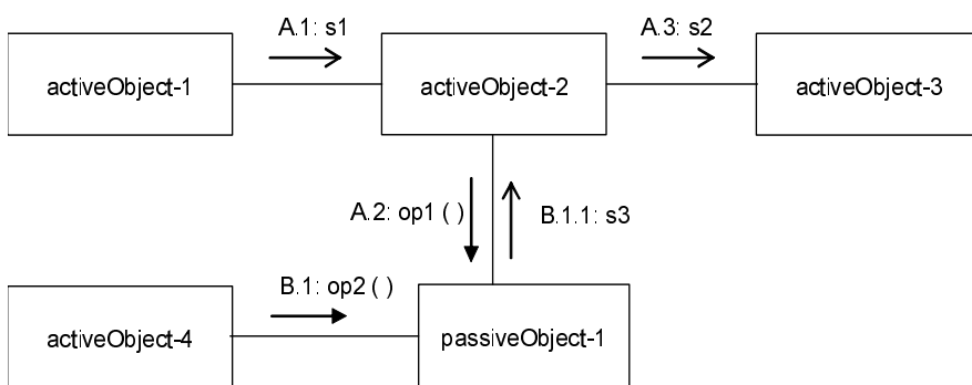
Figure 6.2 - Example illustrating the basic causality model of UML
