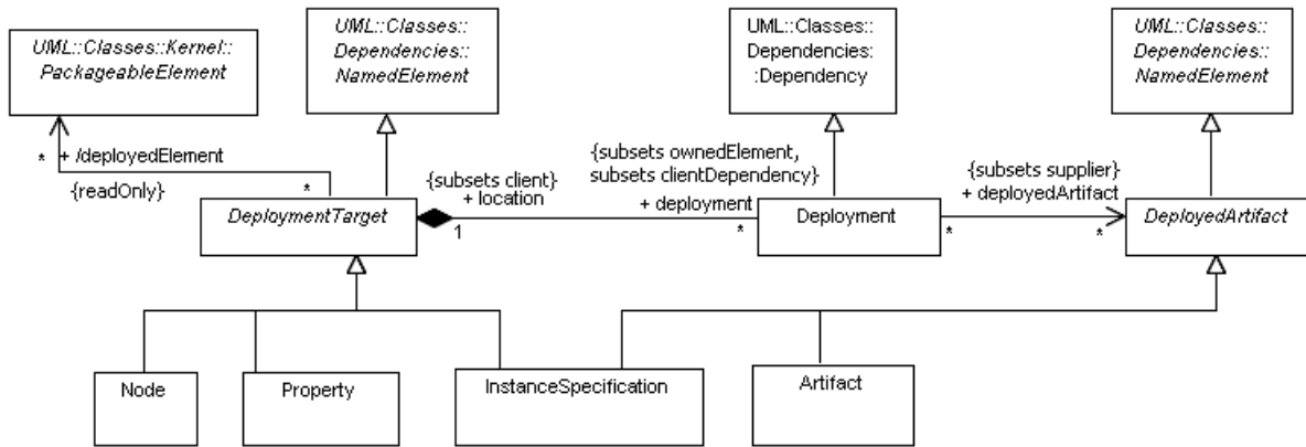
Figure 10.4 - Definition of the Deployment relationship between DeploymentTargets and DeployedArtifacts
