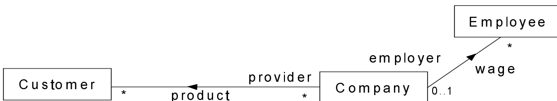
Figure 17.7 - Information Items attached to associations
