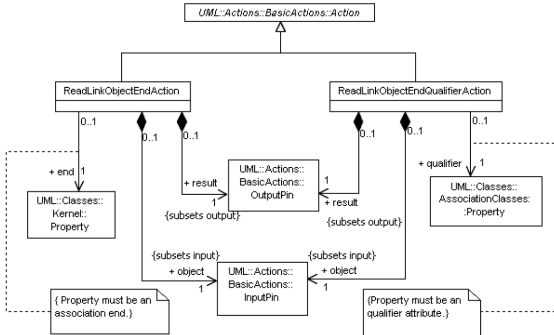
Figure 11.15 - Read link actions (CompleteActions)
