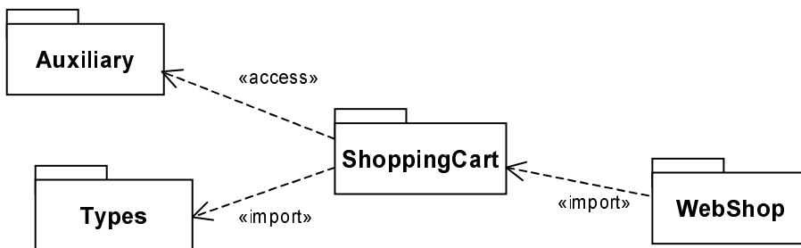
Figure 7.64 - Examples of public and private package imports
