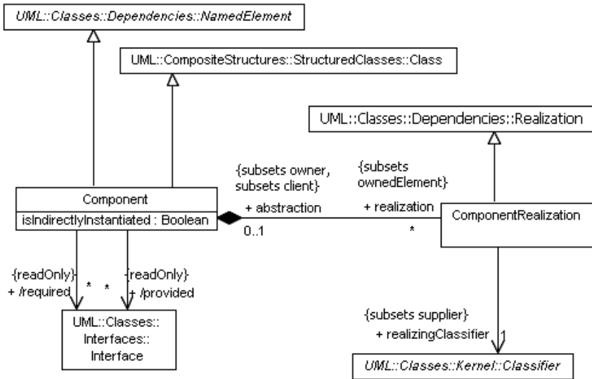
Figure 8.2 - The metaclasses that define the basic Component construct
