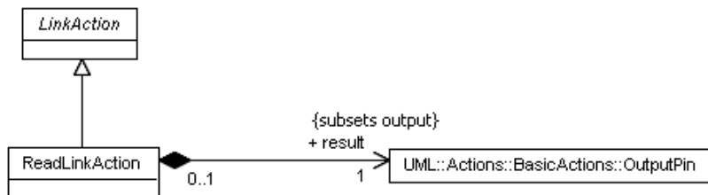
Figure 11.9 - Read link actions
