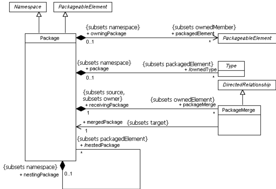
Figure 7.14 - The Packages diagram of the Kernel package
