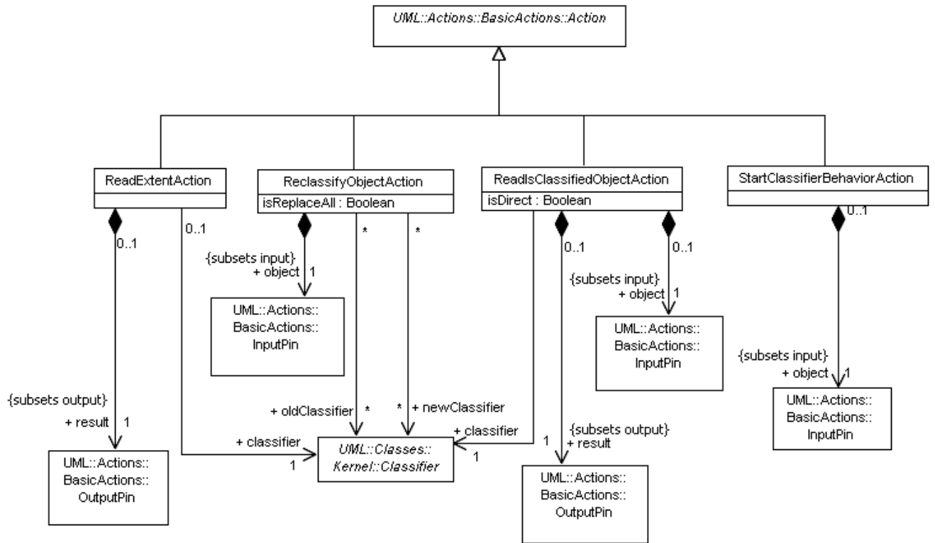
Figure 11.13 - Object actions (CompleteActions)
