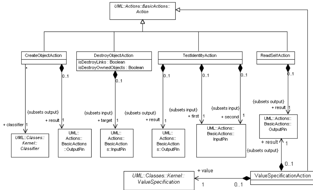
Figure 11.6 - Object actions
