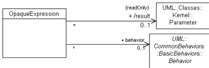
Figure 13.7 - Expression
