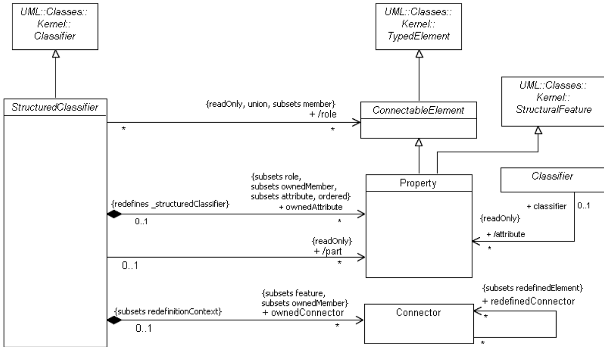
Figure 9.2 - Structured classifier
