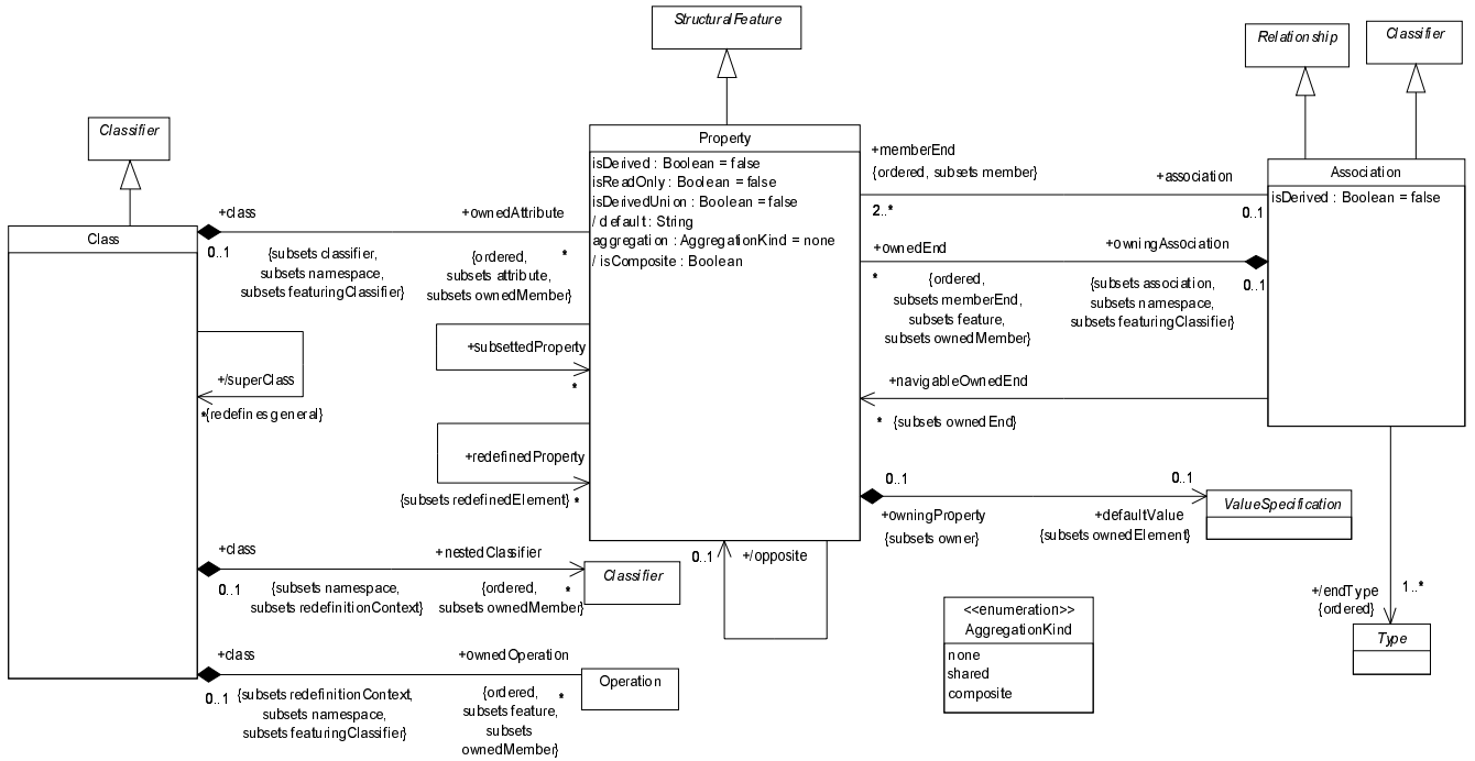
Figure 7.12 - Classes diagram of the Kernel package
